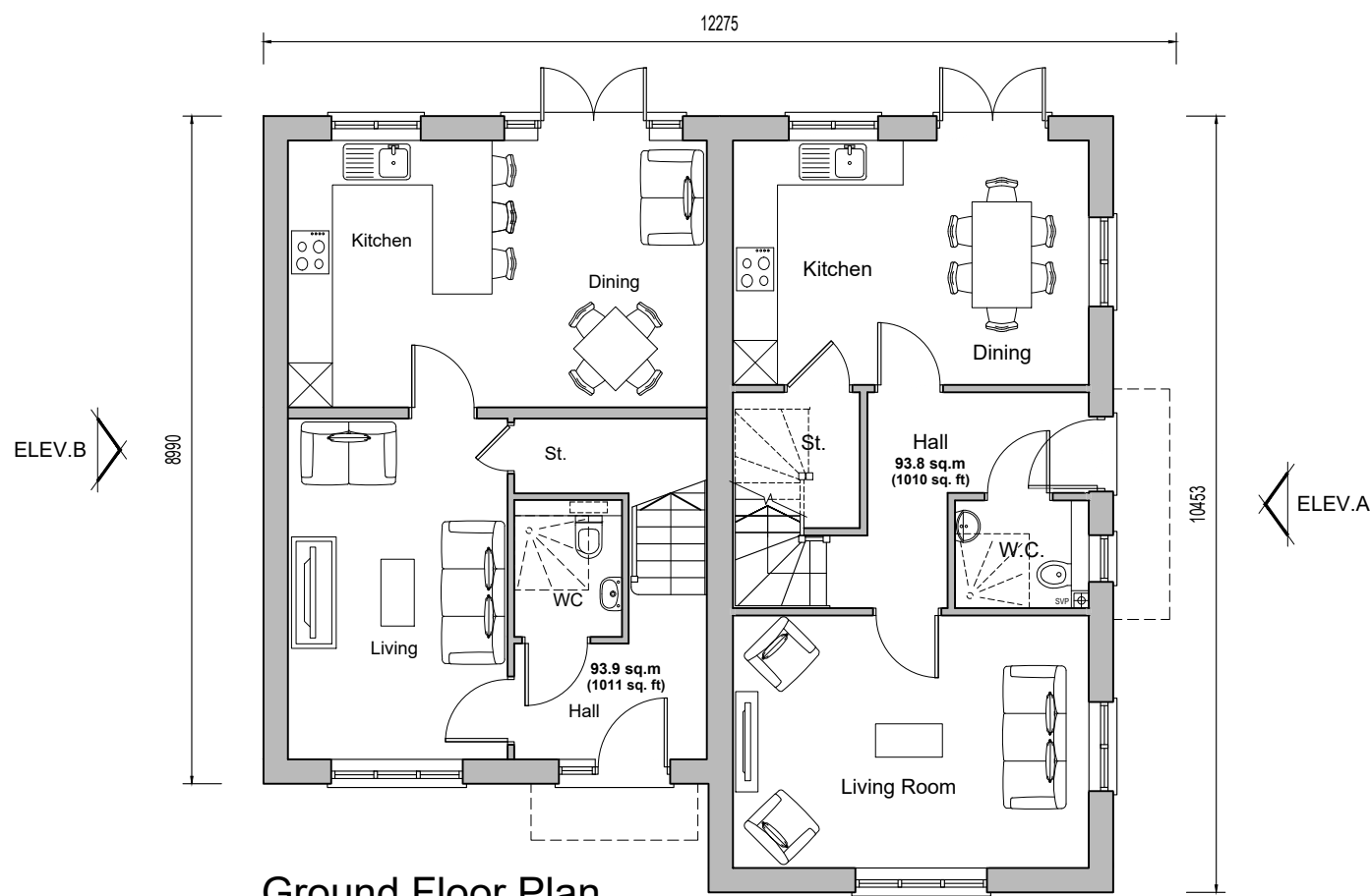
Ground Floor Plan Plots 419-420 Plots 421-422 (handed)
