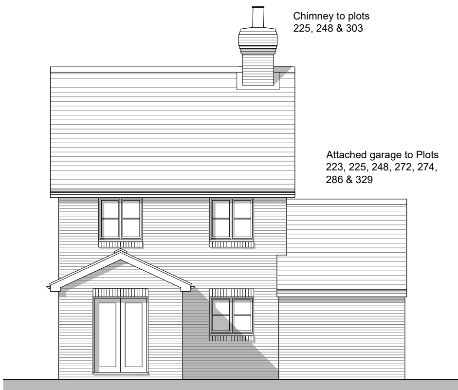
Rear Elevation
