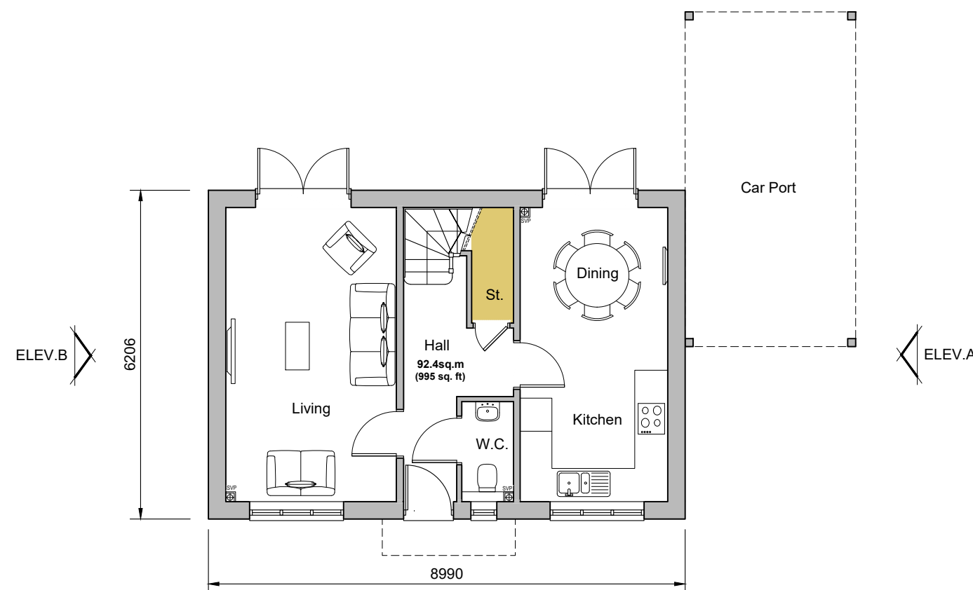
Ground Floor Plan Plot 213
