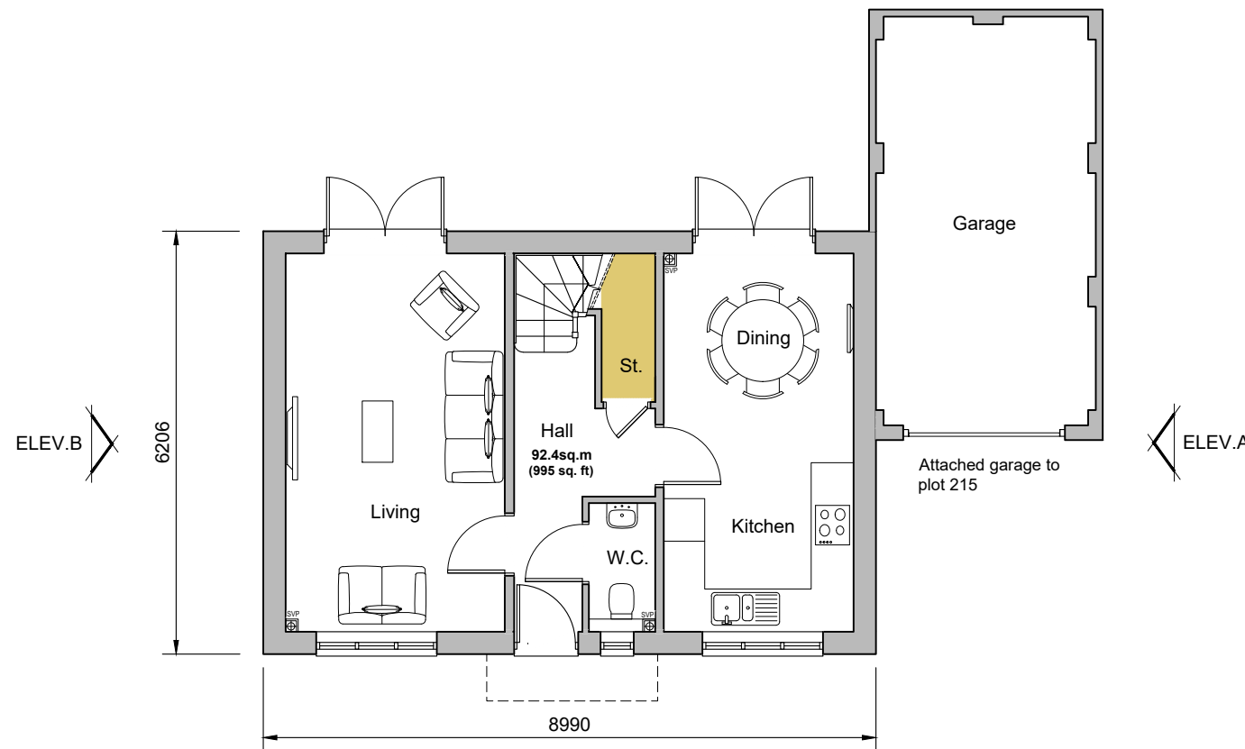
Ground Floor Plan Plots 197, 215 & 231
