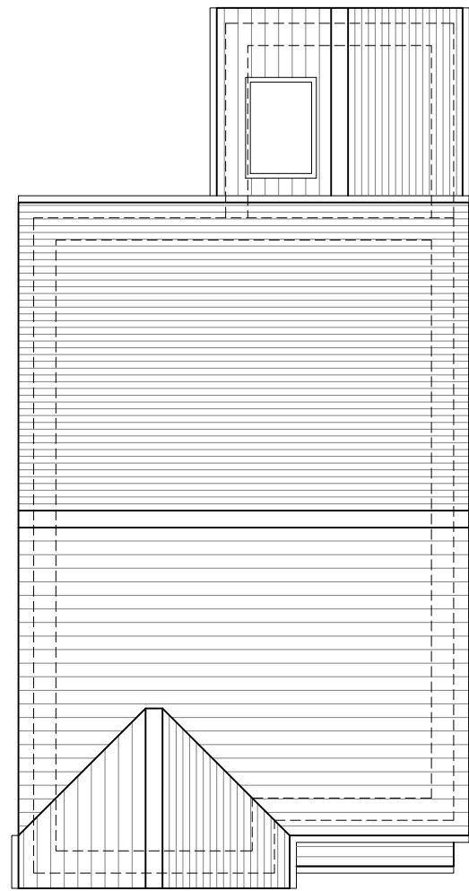
Roof Plan
