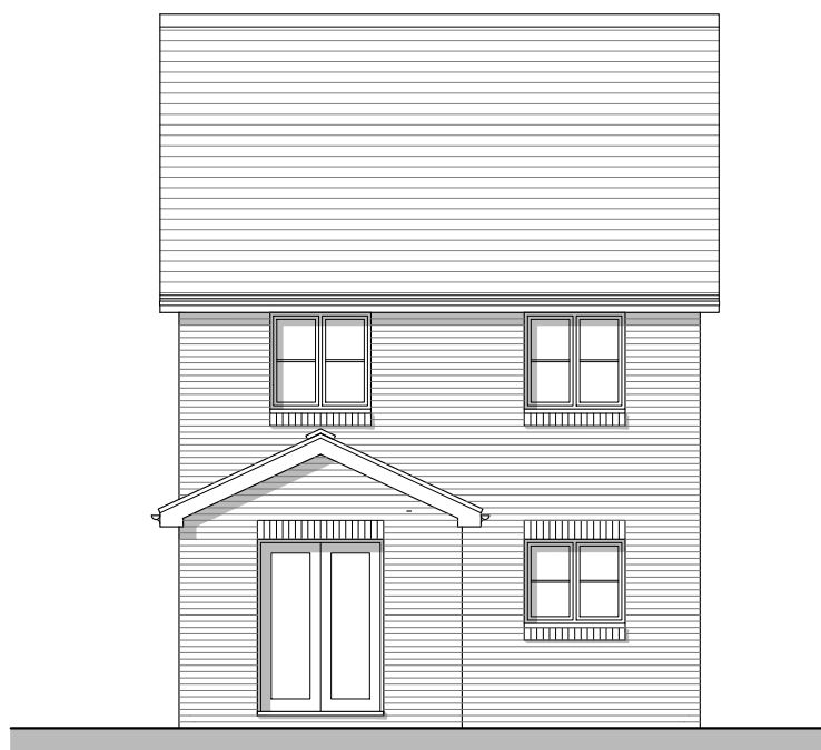
Rear Elevation
