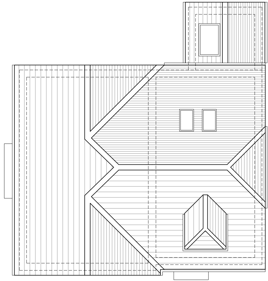
Roof Plan
