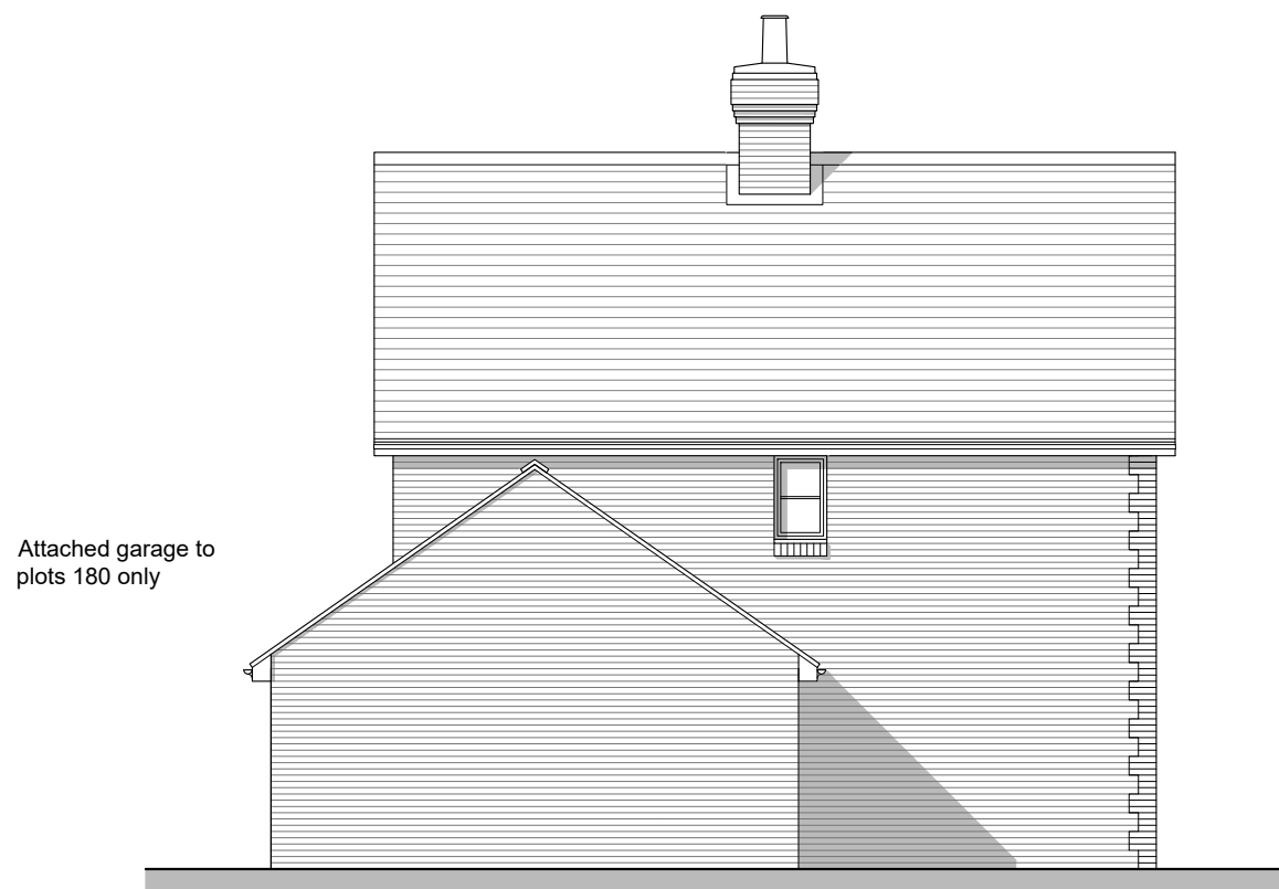
Rear Elevation Plots 180, 291 Plots 255, 330 (handed)
