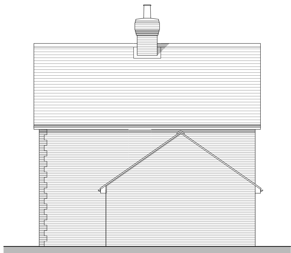
Rear Elevation Plot 235
