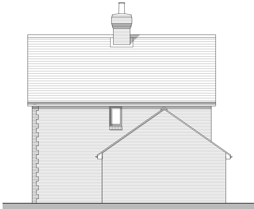
Rear Elevation Plot 143
