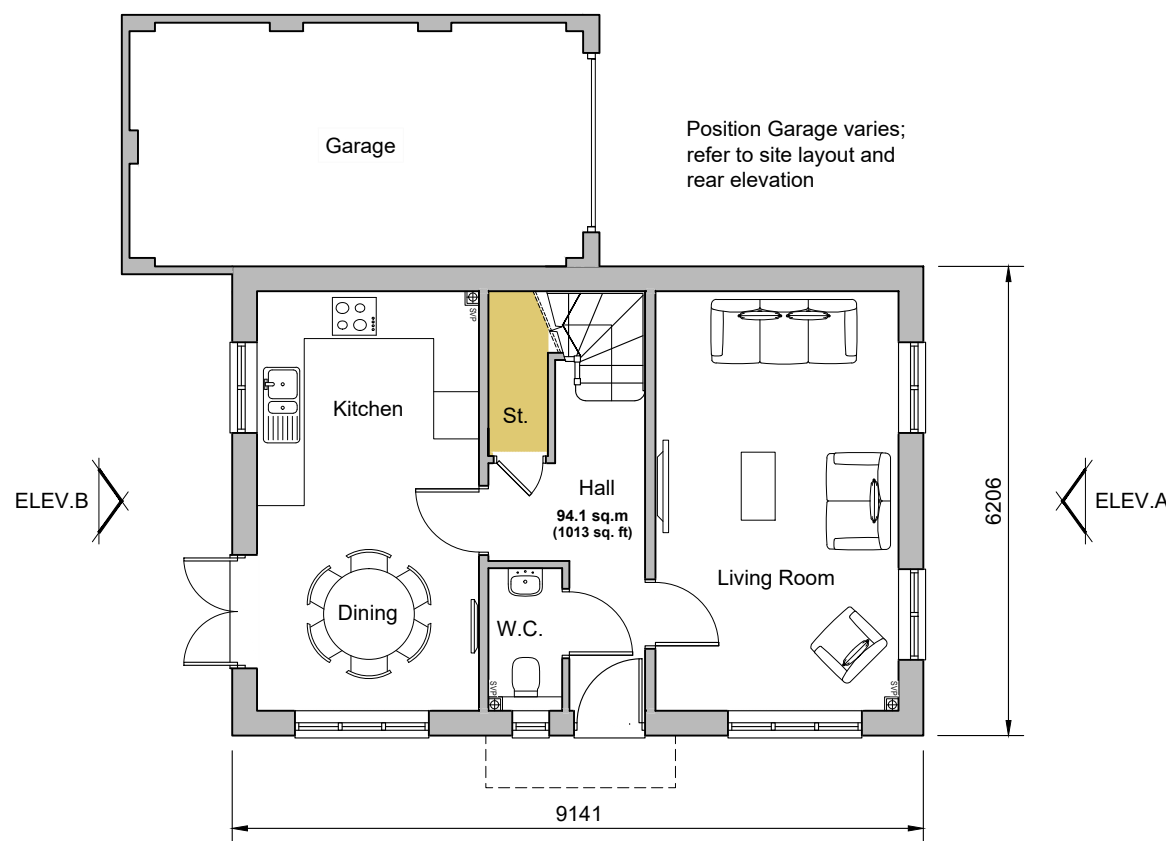
Ground Floor Plan Plots 3, 143
