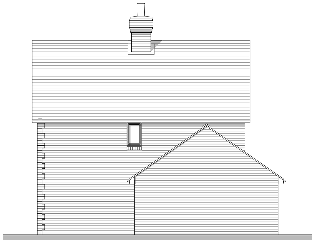
Rear Elevation Plot 3
