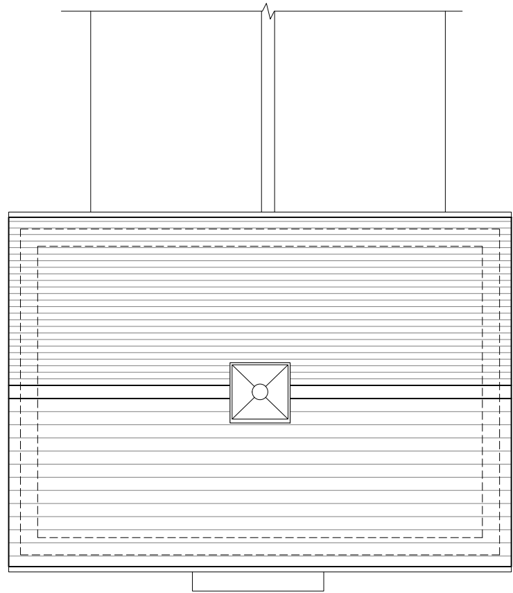
Roof Plan
