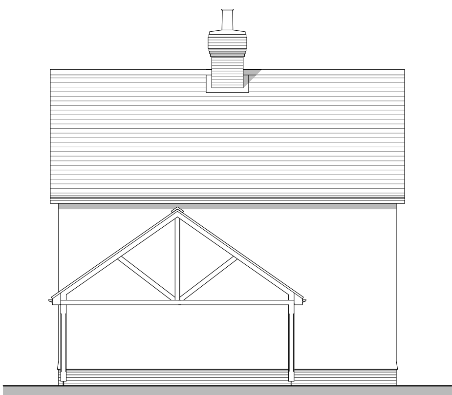
Rear Elevation Plot 75 (handed)
