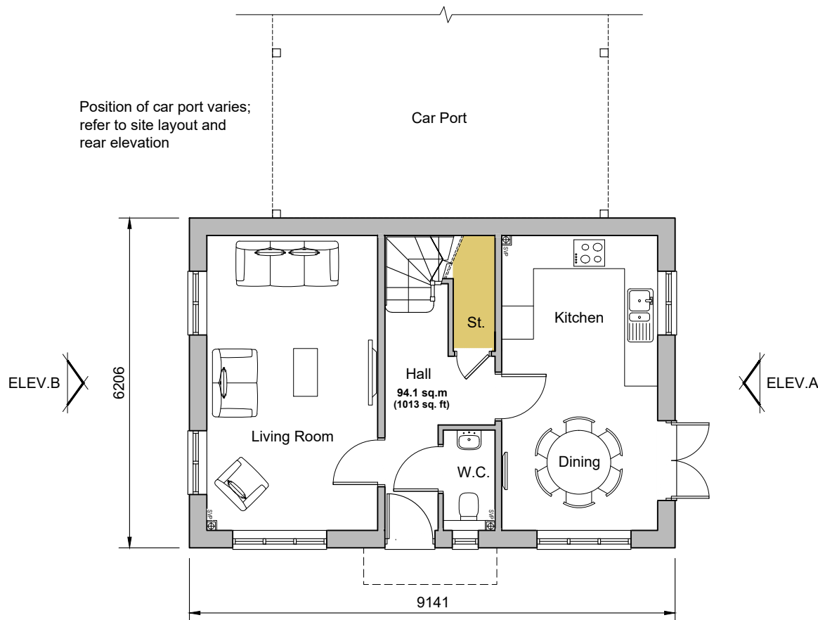
Ground Floor Plan Plot 76 Plot 75 (handed)
