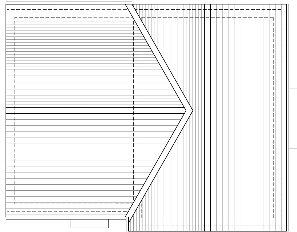
Roof Plan
