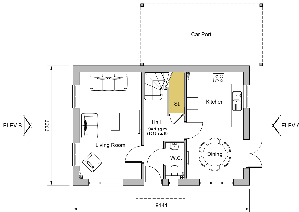
Ground Floor Plan Plot 206
