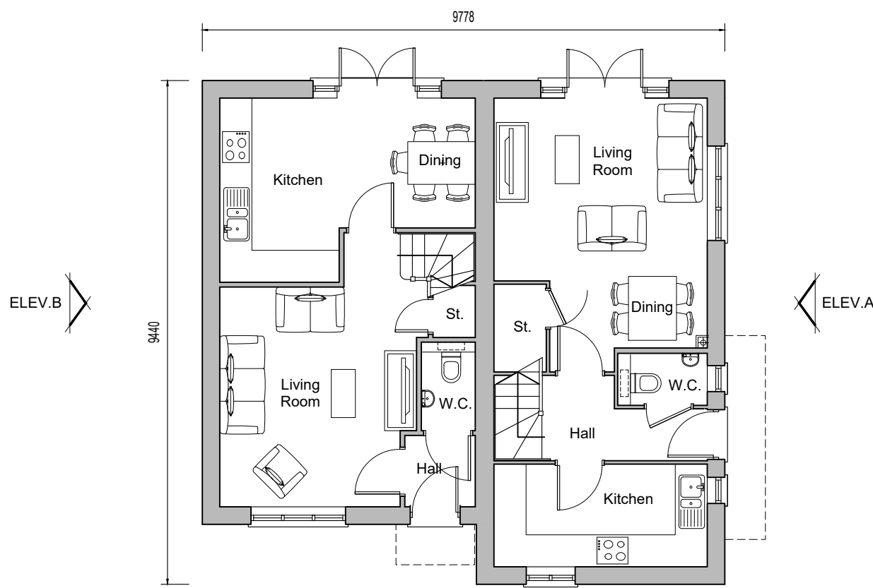
Ground Floor Plan Plots 433-434 Plots 402-403 (handed)
