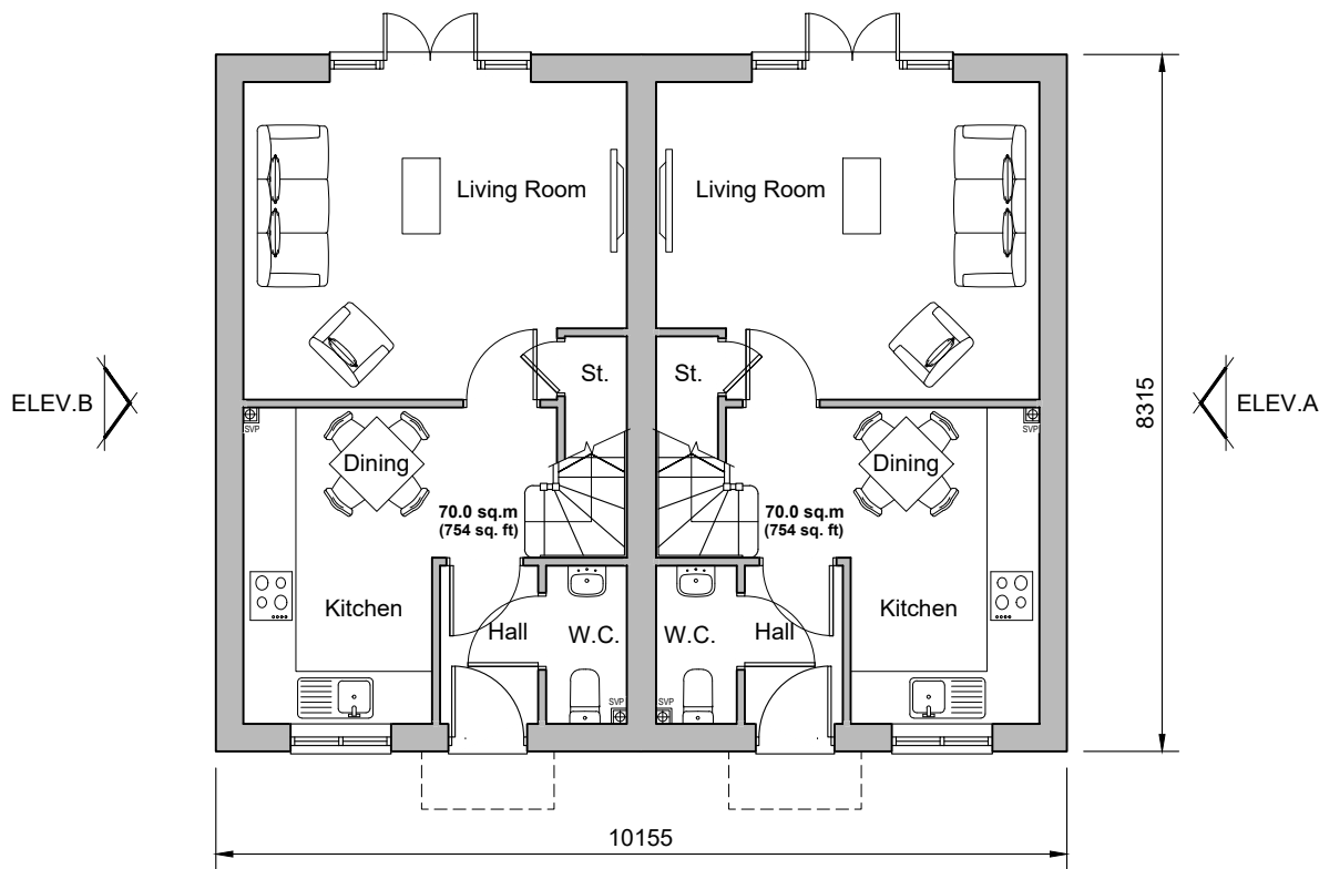
Ground Floor Plan Plots 207-208 & 209-210
