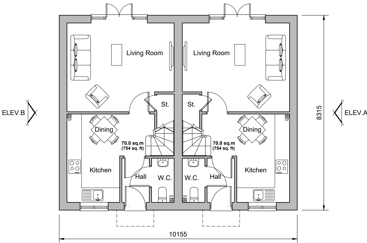
Ground Floor Plan Plots 131-132
