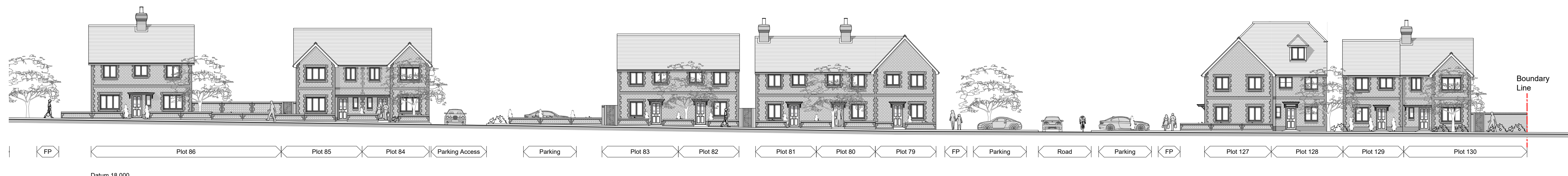
Street Scene D-D
