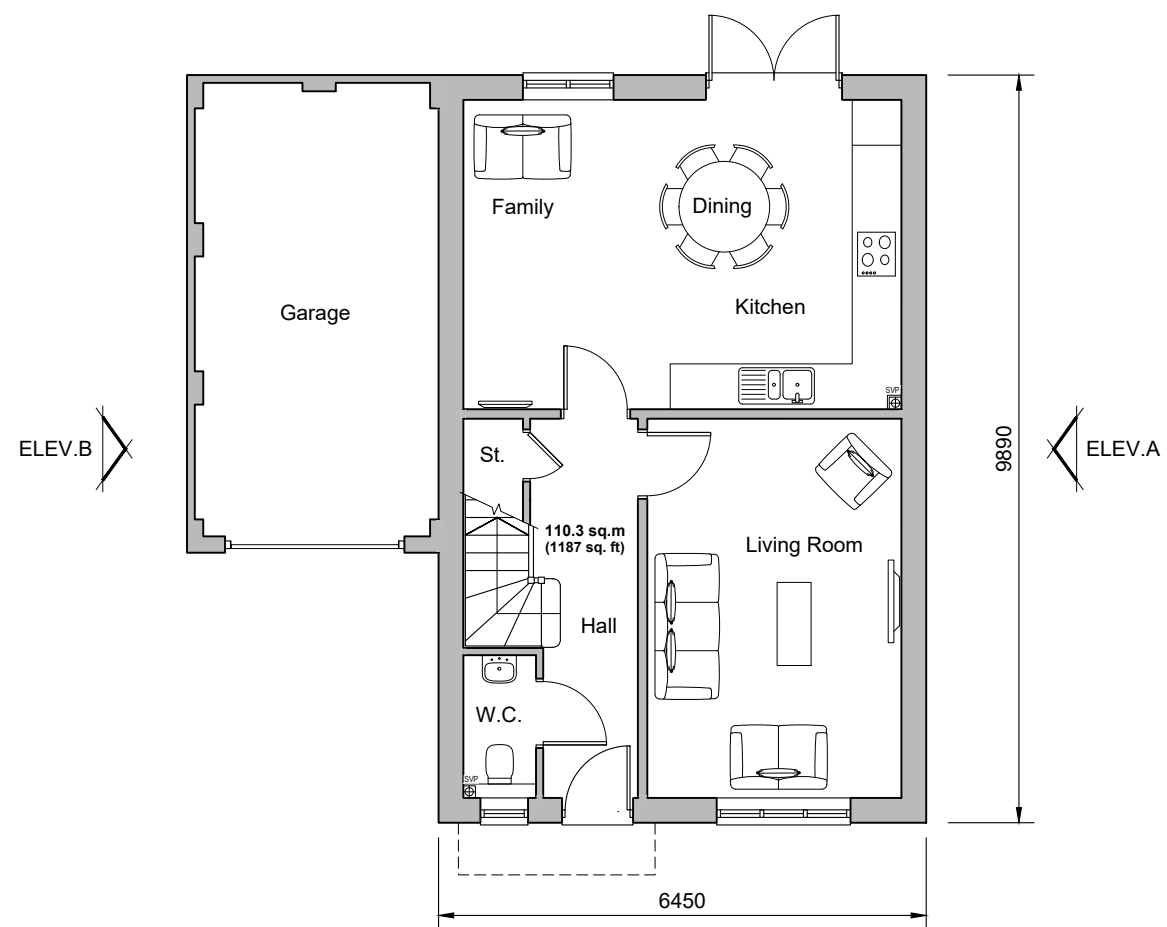
Ground Floor Plan Plot 151
