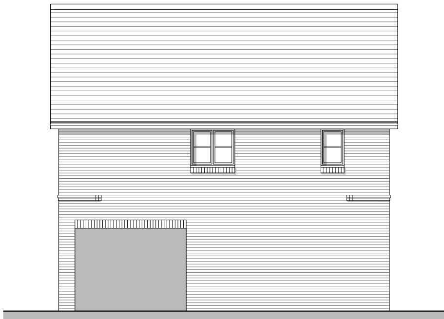
Rear Elevation
