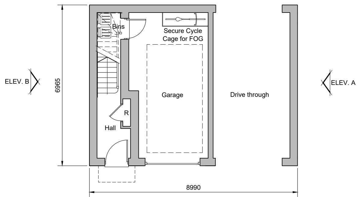
Ground Floor Plan Plot 125
