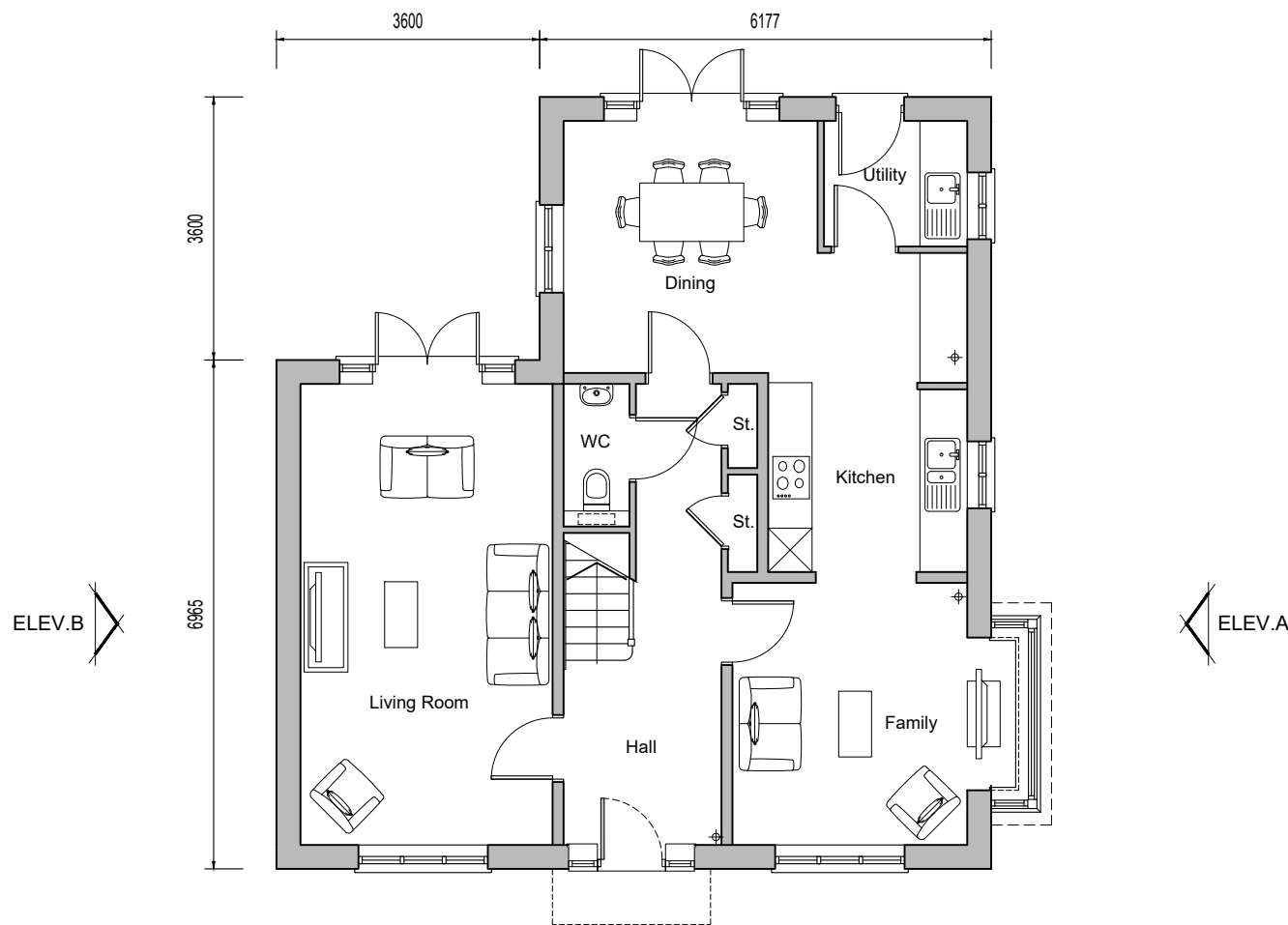
Ground Floor Plan Plot 503 Plots 477 (handed)
