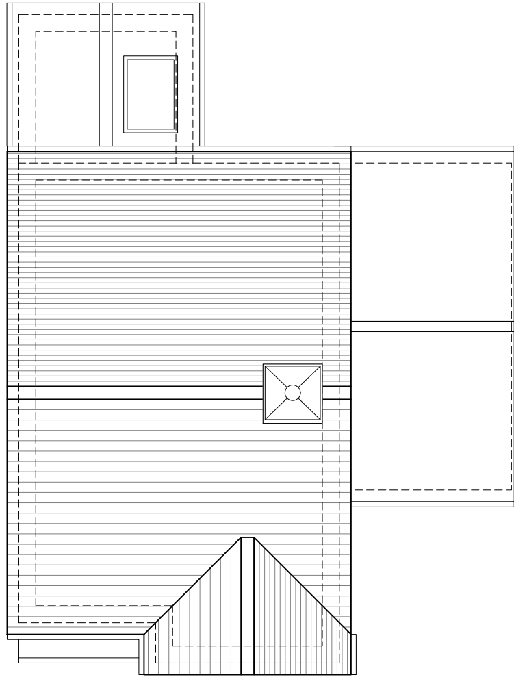
Roof Plan
