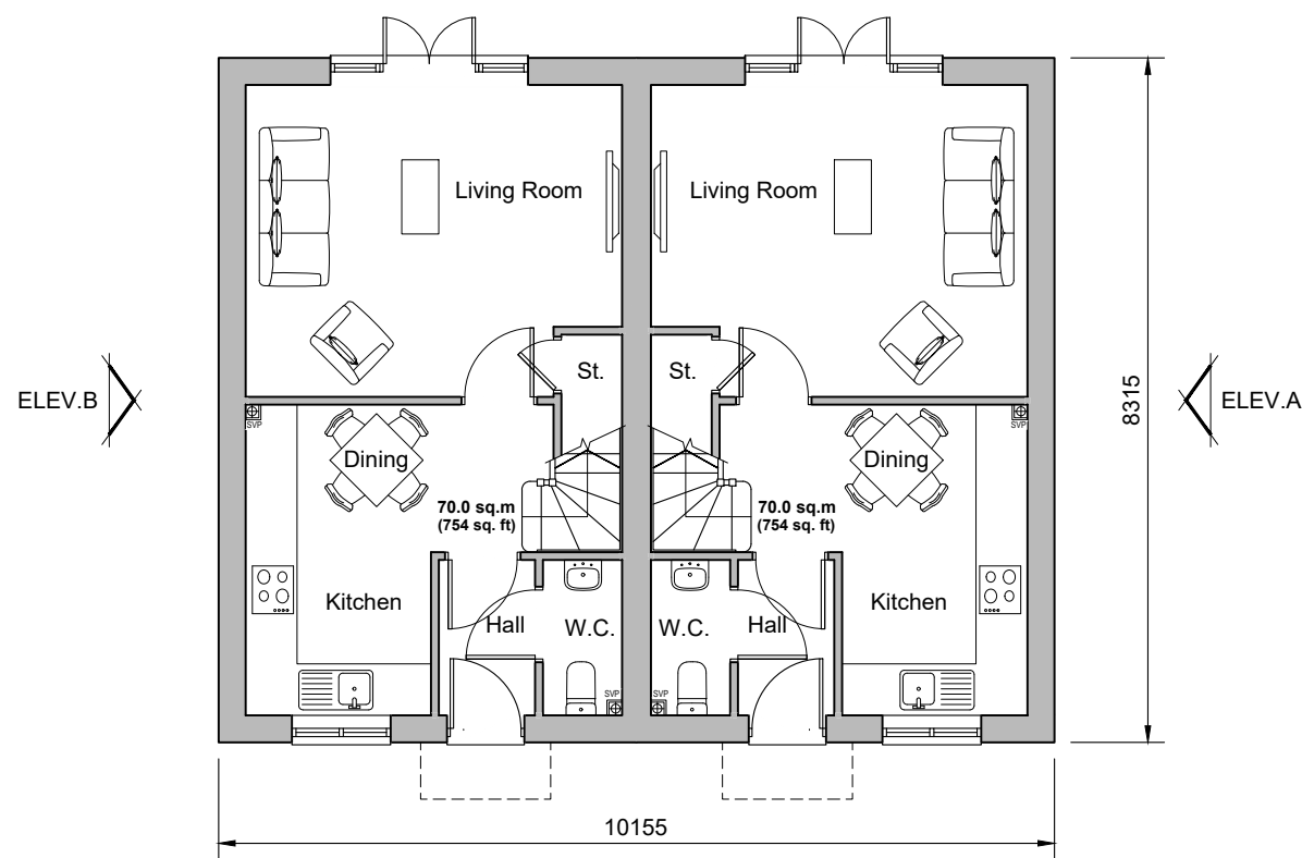
Ground Floor Plan Plots 165-166, 212-213 & 214-215
