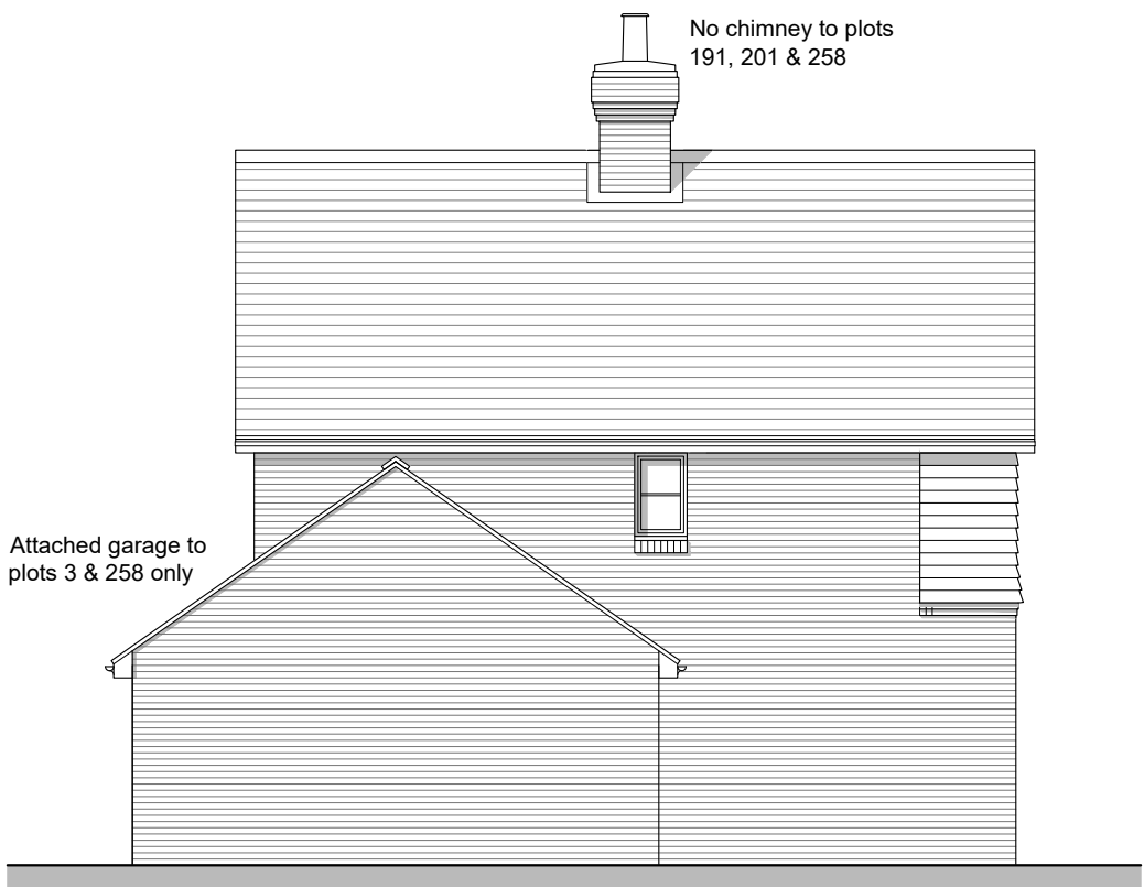
Rear Elevation
