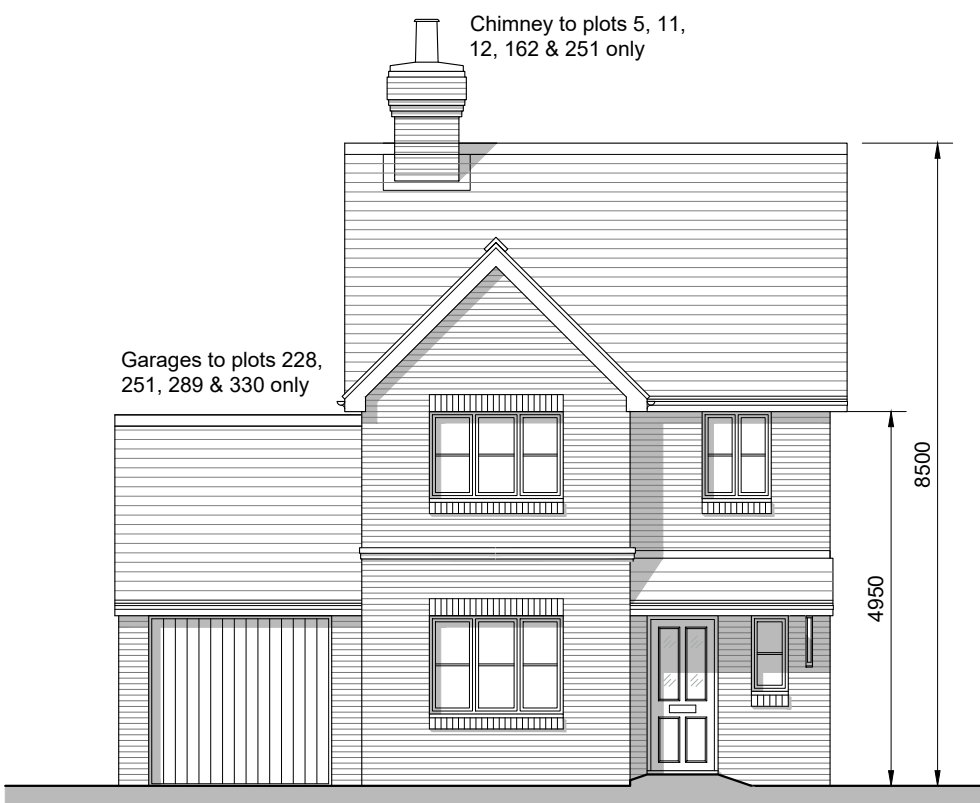
Front Elevation
