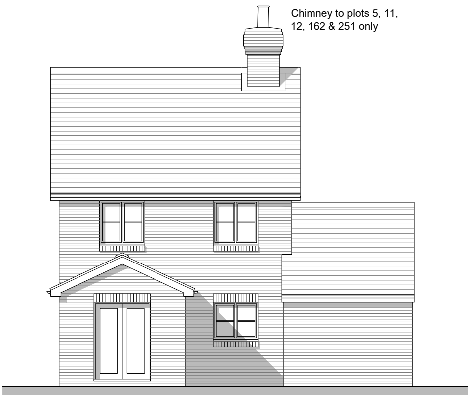
Rear Elevation
