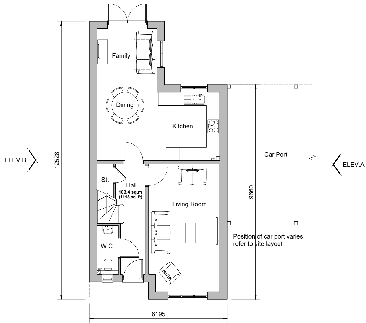
Ground Floor Plan Plots 51 & 159
