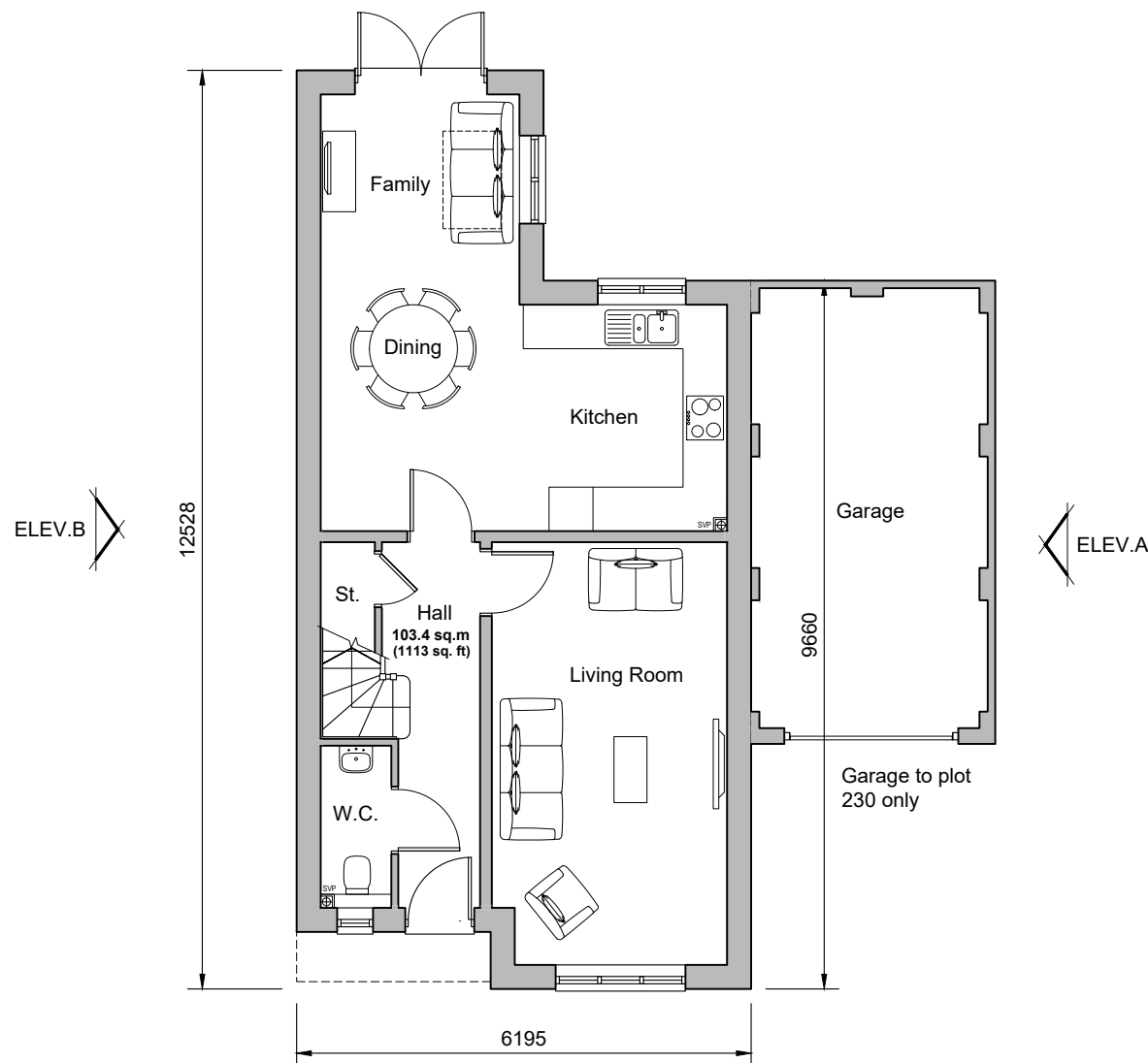
Ground Floor Plan Plots 230 & 304
