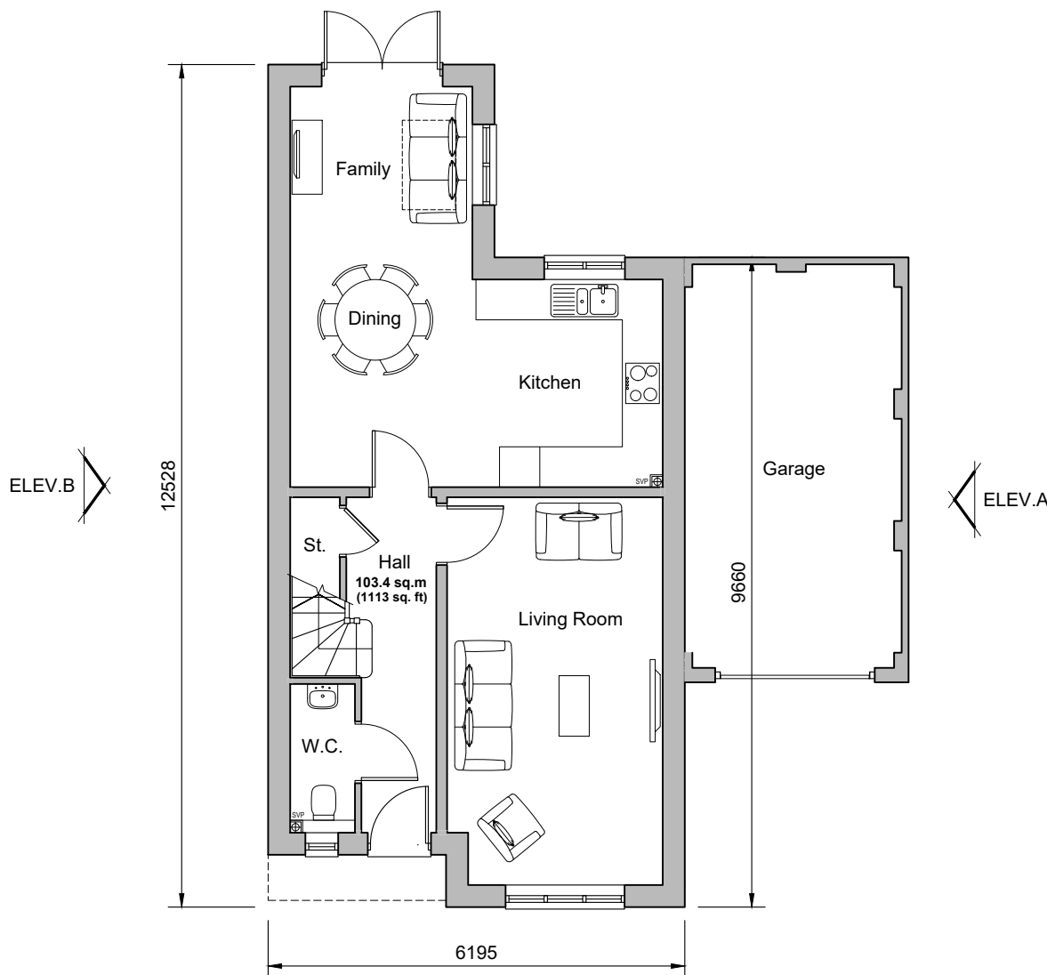
Ground Floor Plan Plot 52
