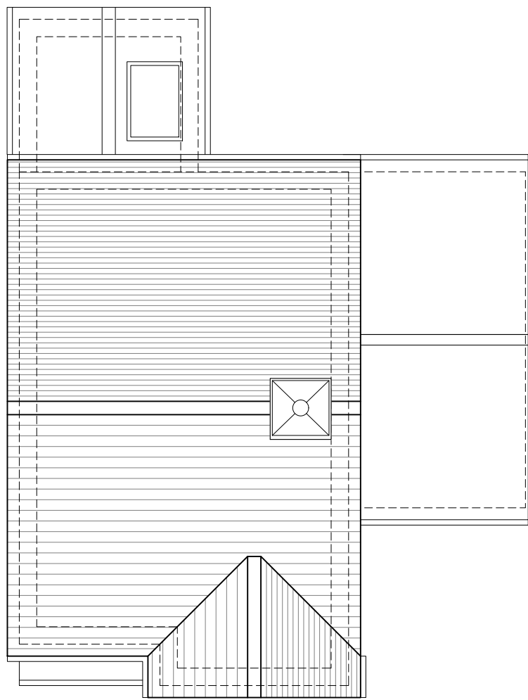
Roof Plan
