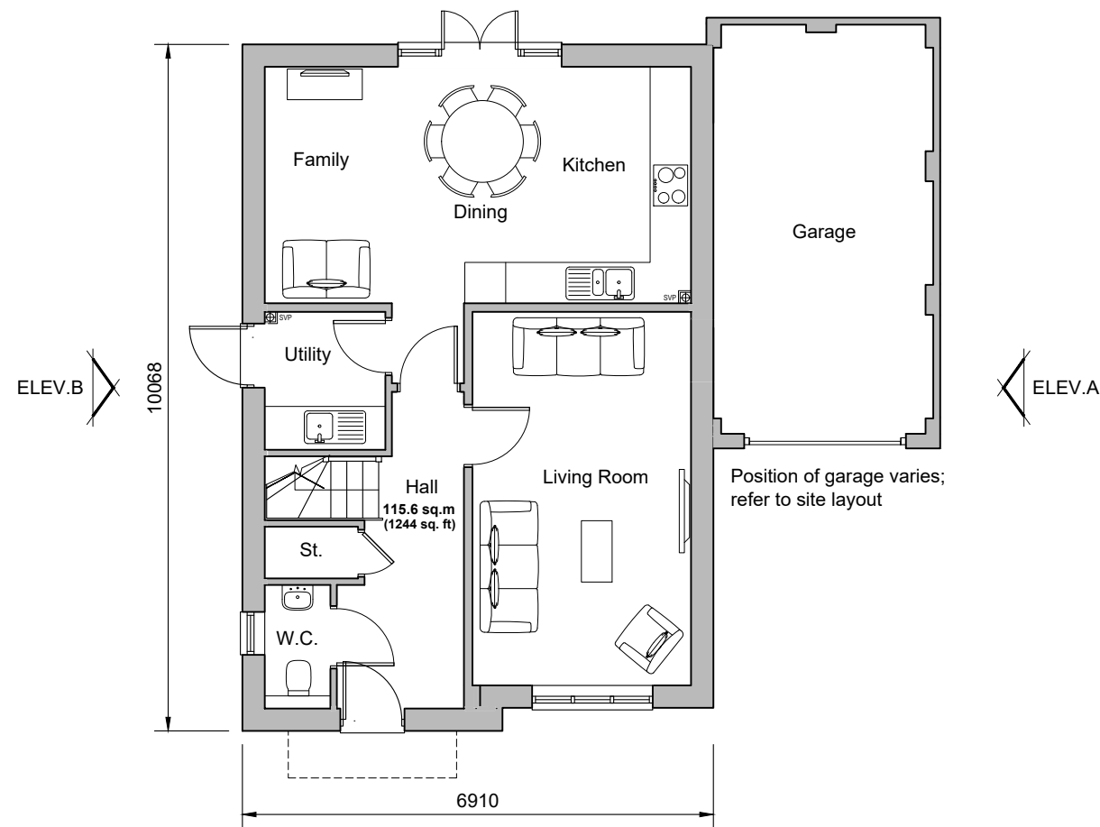
Ground Floor Plan Plots 229 & 234
