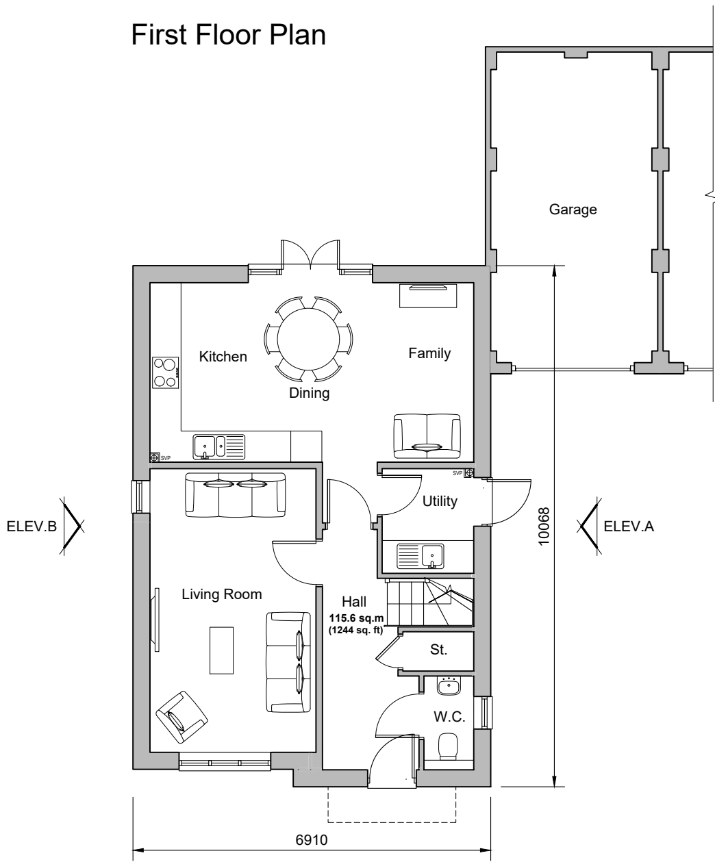
Ground Floor Plan Plot 4
