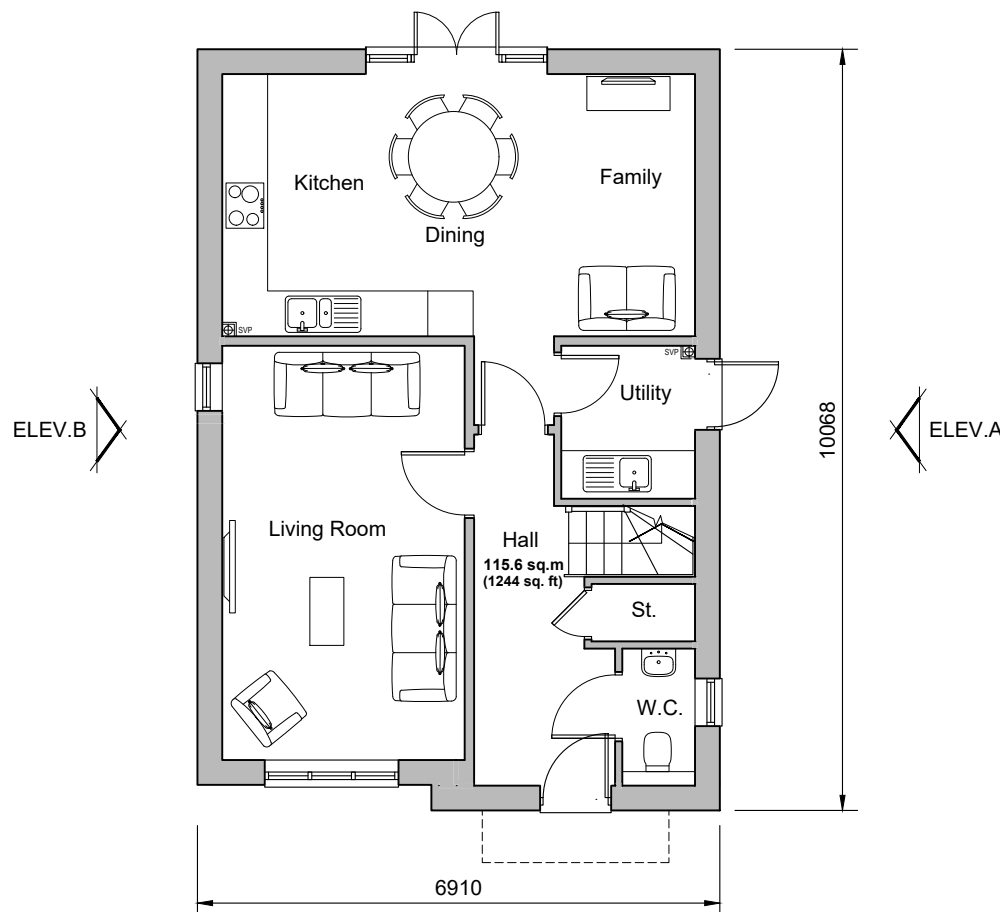
Ground Floor Plan Plot 180
