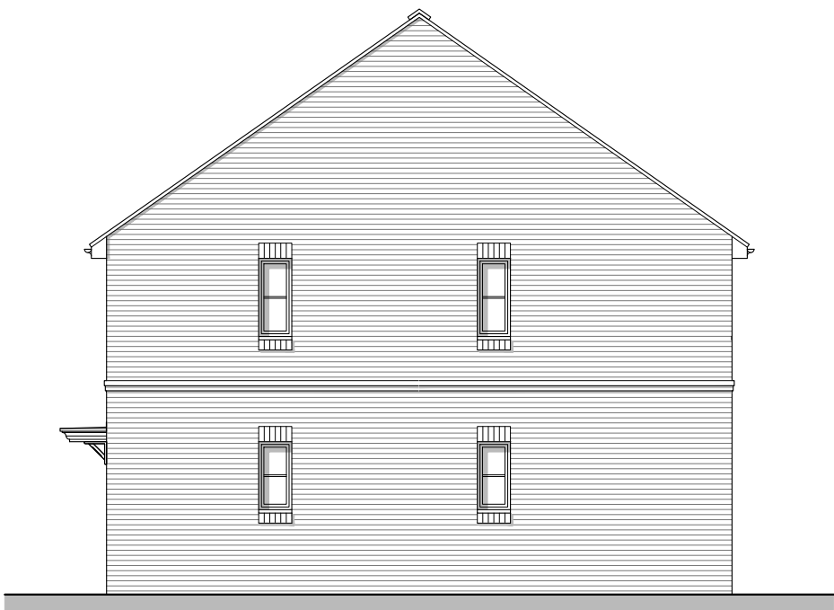
Side Elevation A Plot 177
