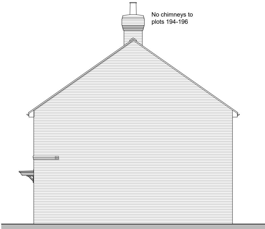
Side Elevation A Plots 36, 39, 42, 45 & 194
