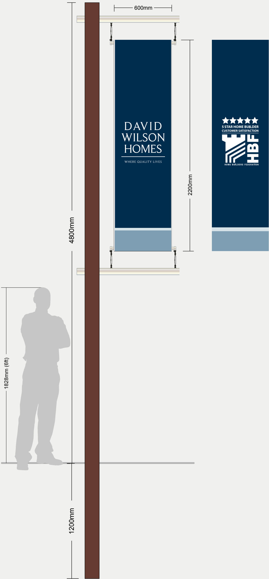
DWH Static Banner Flag Sign Wood effect Square Aluminium Post 6000mm x 150mm x 150mm
