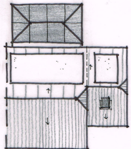
ROOF PLAN 1:200
