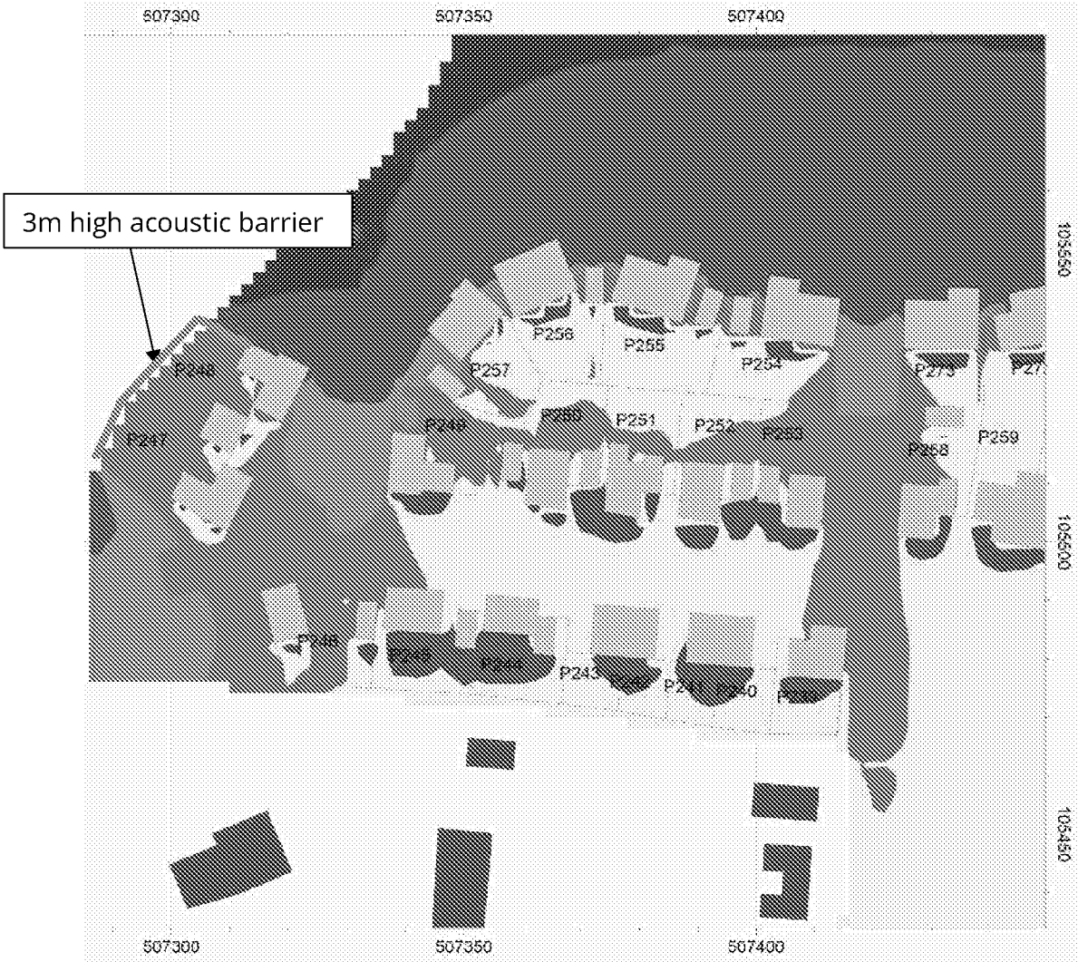
Figure C3: Daytime Noise Contours with 3m Acoustic Barrier
