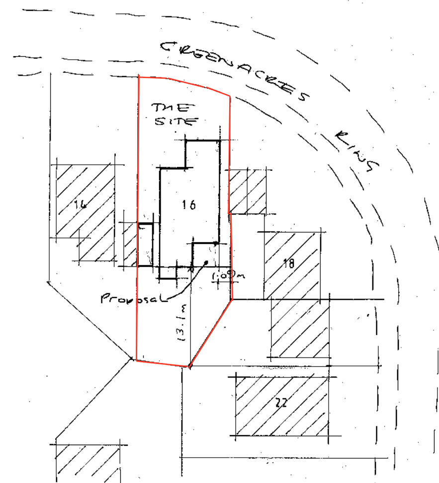
Block plan 1:500
