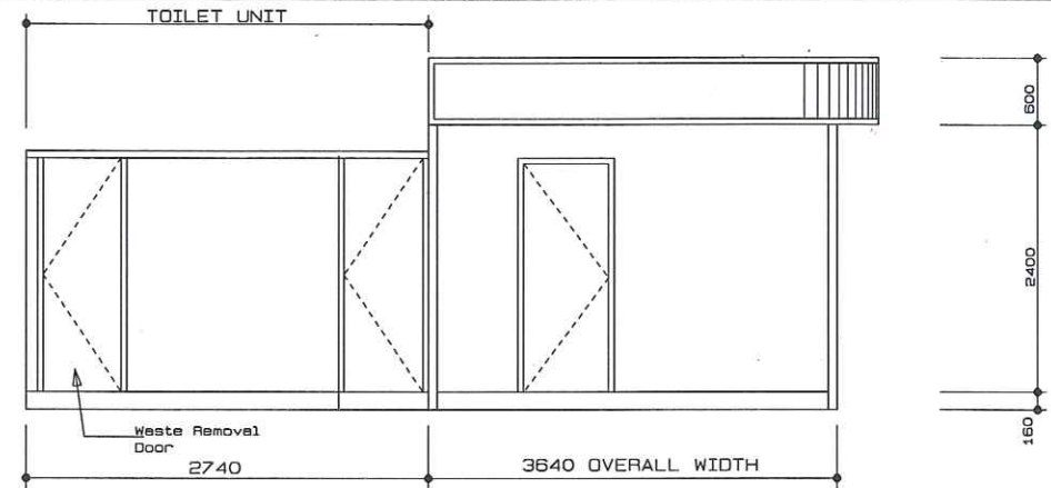
GABLE ELEVATION ON ARROW A
