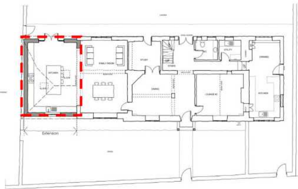
Proposed extension: main elevation and floor plan
