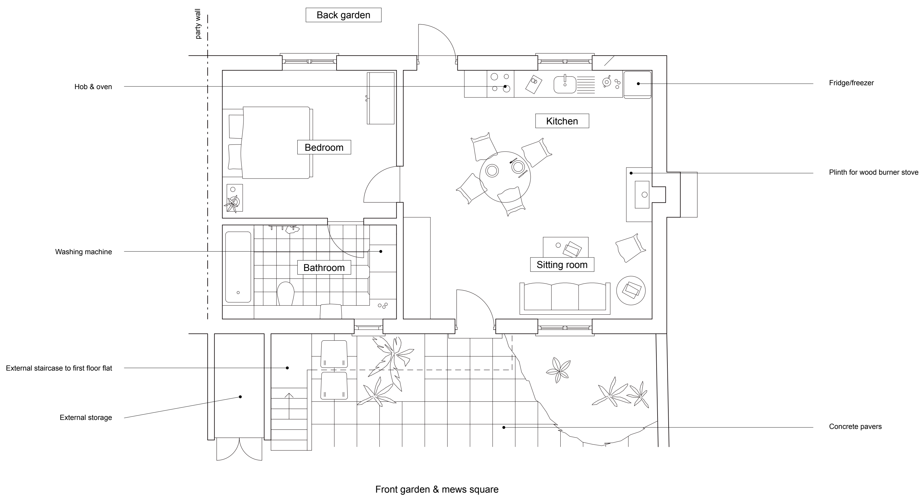
C Terrace C (flat) - Ground floor plan
