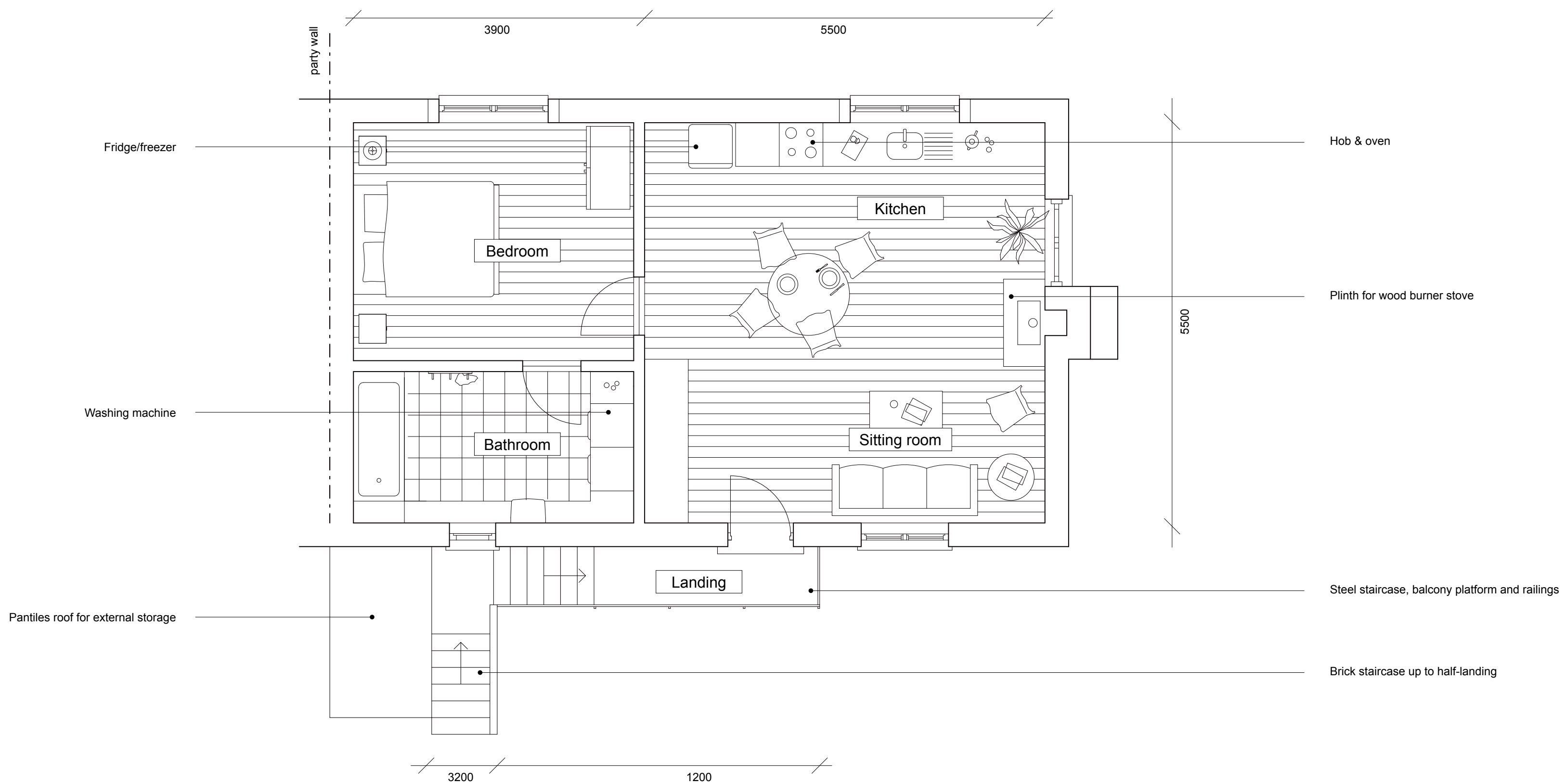
C Terrace C (flat) - First floor plan
