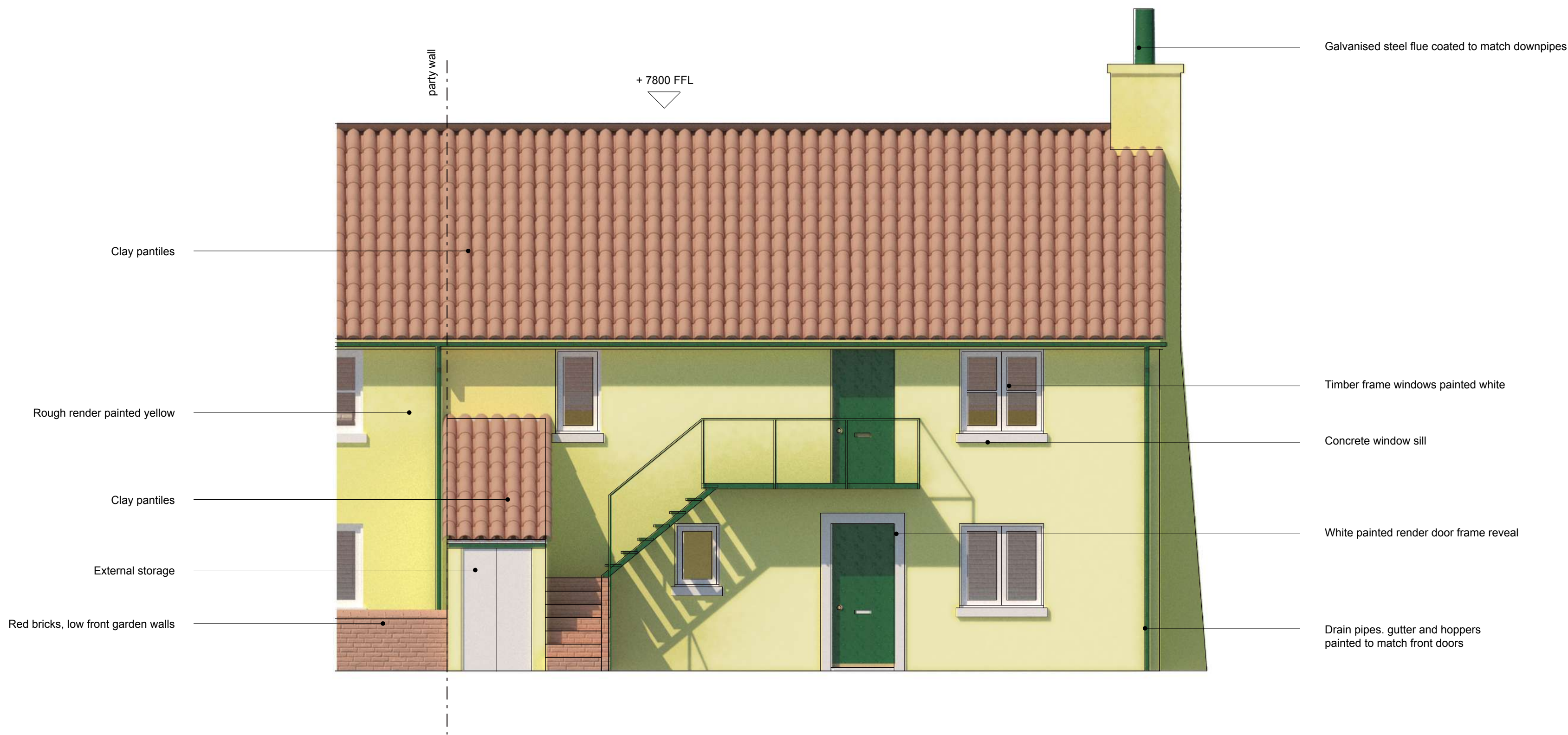
C Terrace C (flats) - Front elevation (East)
