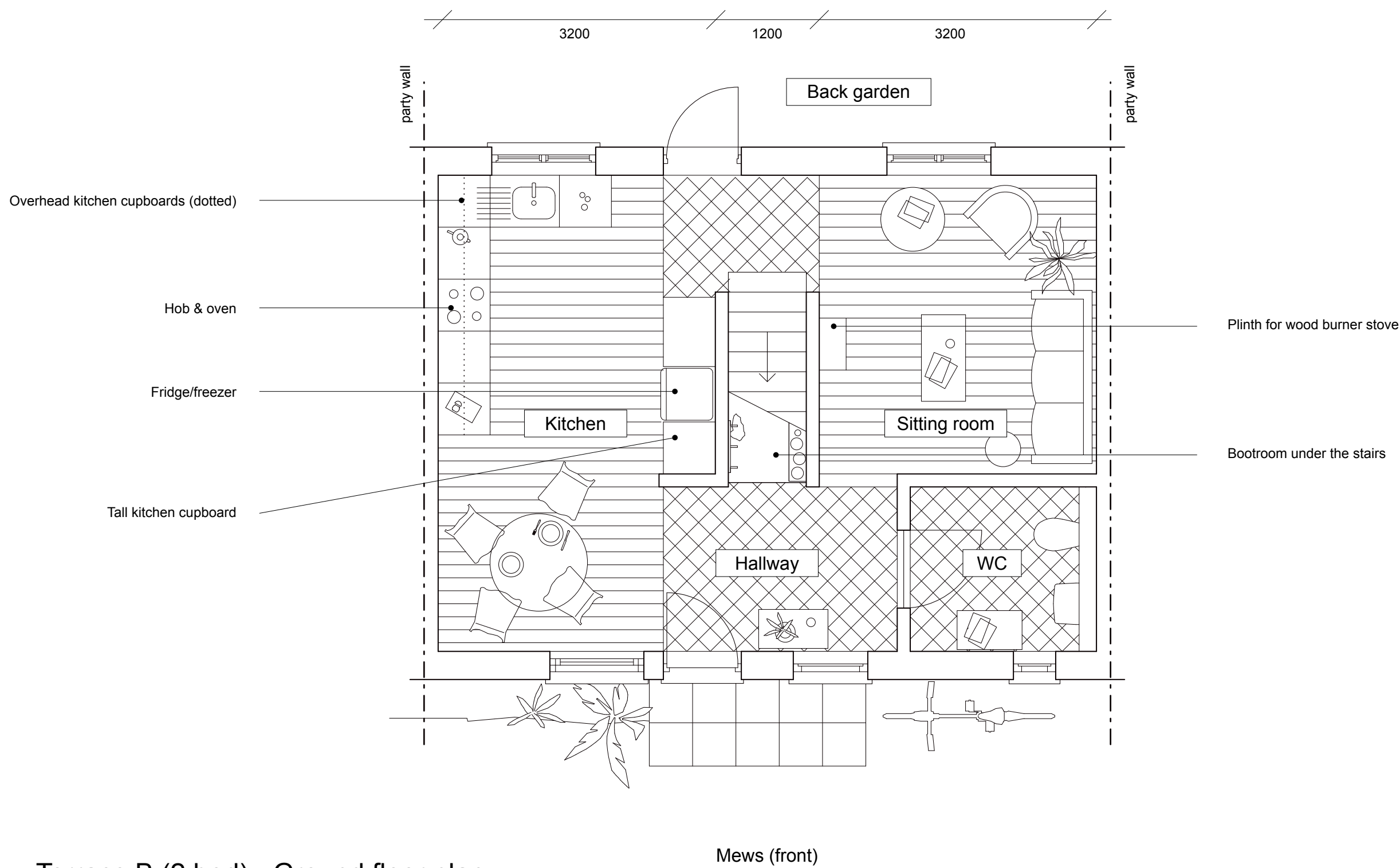
B Terrace B (2 bed) - Ground floor plan
