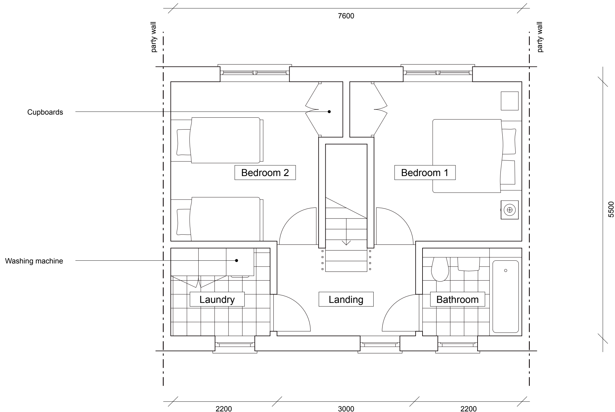
B Terrace B (2 bed) - First floor plan
