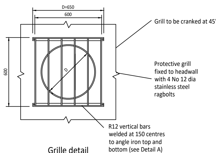
Grille detail
