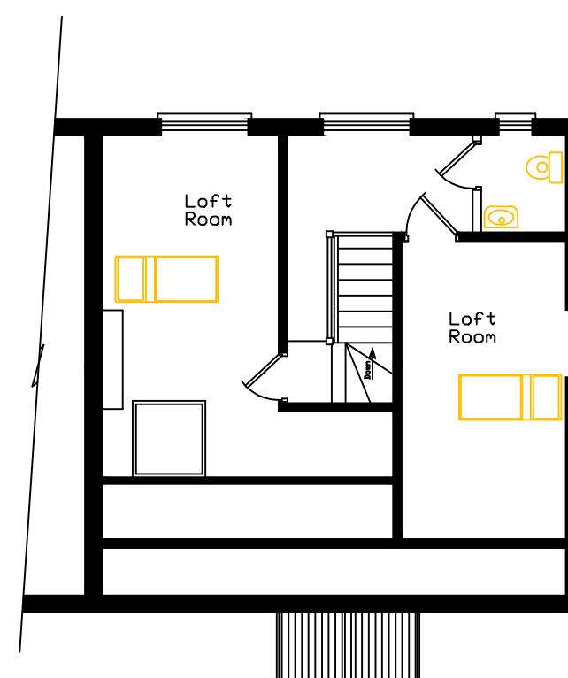
Proposed Loft Room Plan
