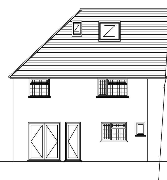
Existing West Elevation
