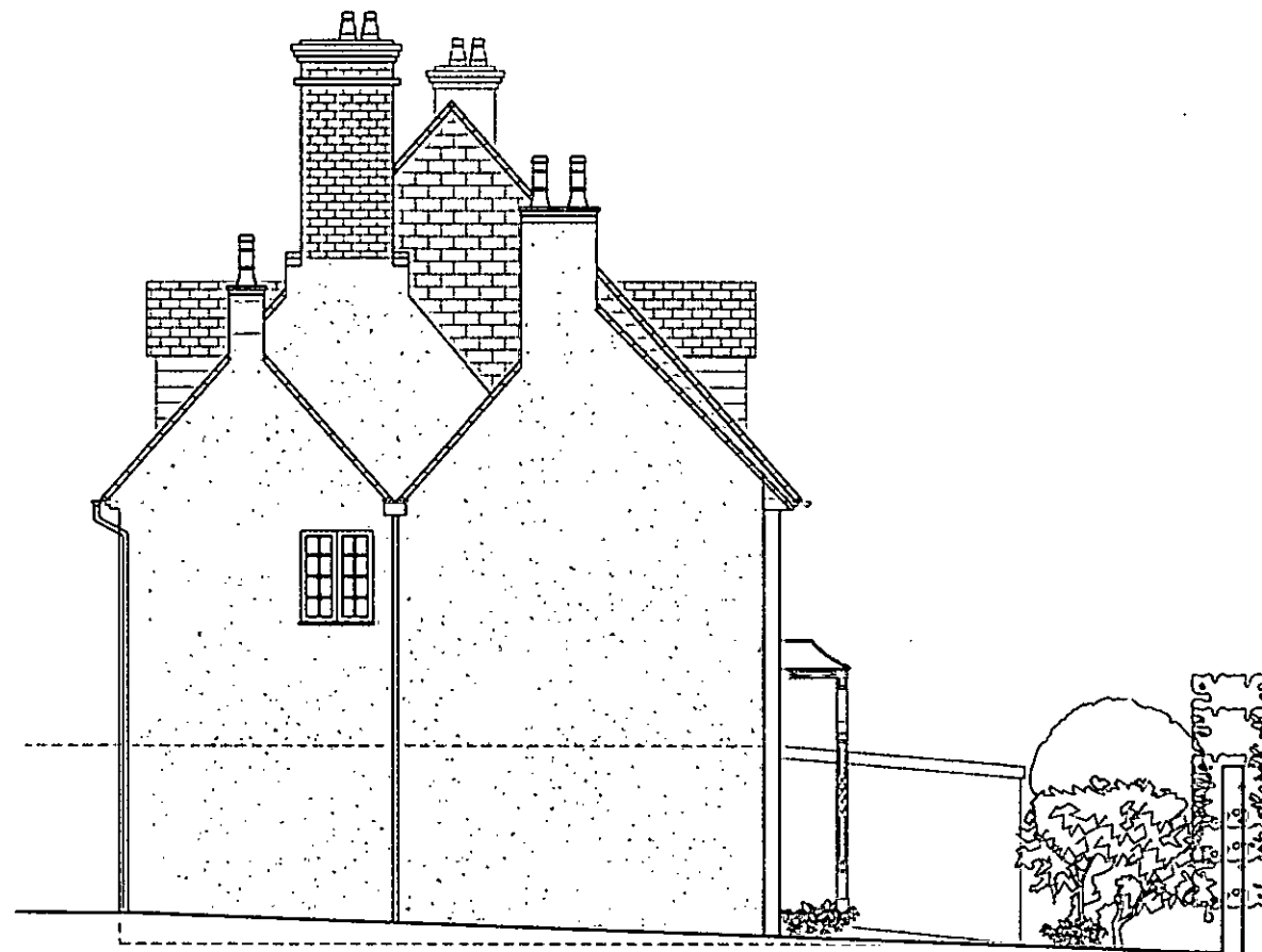
SIDE ELEVATION
