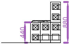
SIDE VIEW BENCHES
