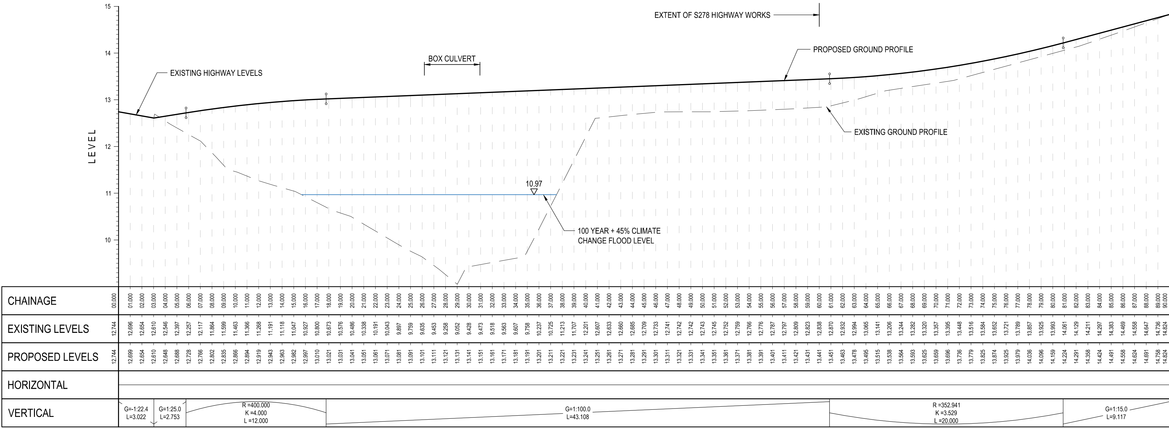
PROPOSED ACCESS CENTRELINE SCALE: H 1:200, V 1:50. DATUM: 9.000
