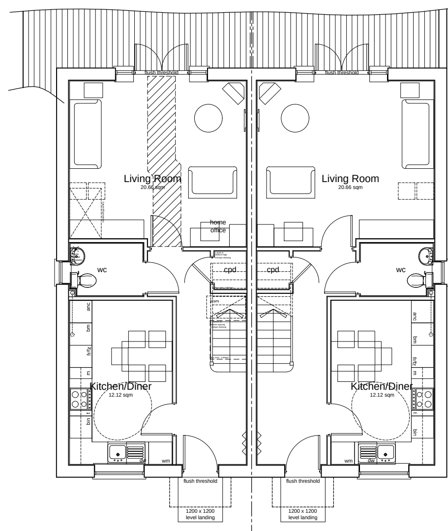
Plot 21 - 3 Bed 5p House
