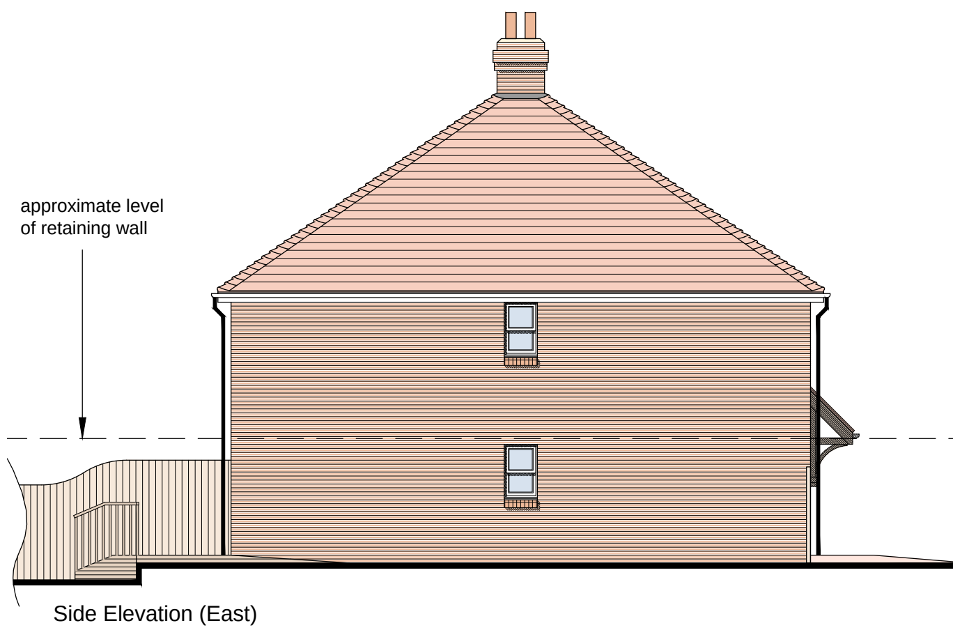
Side Elevation (East)
