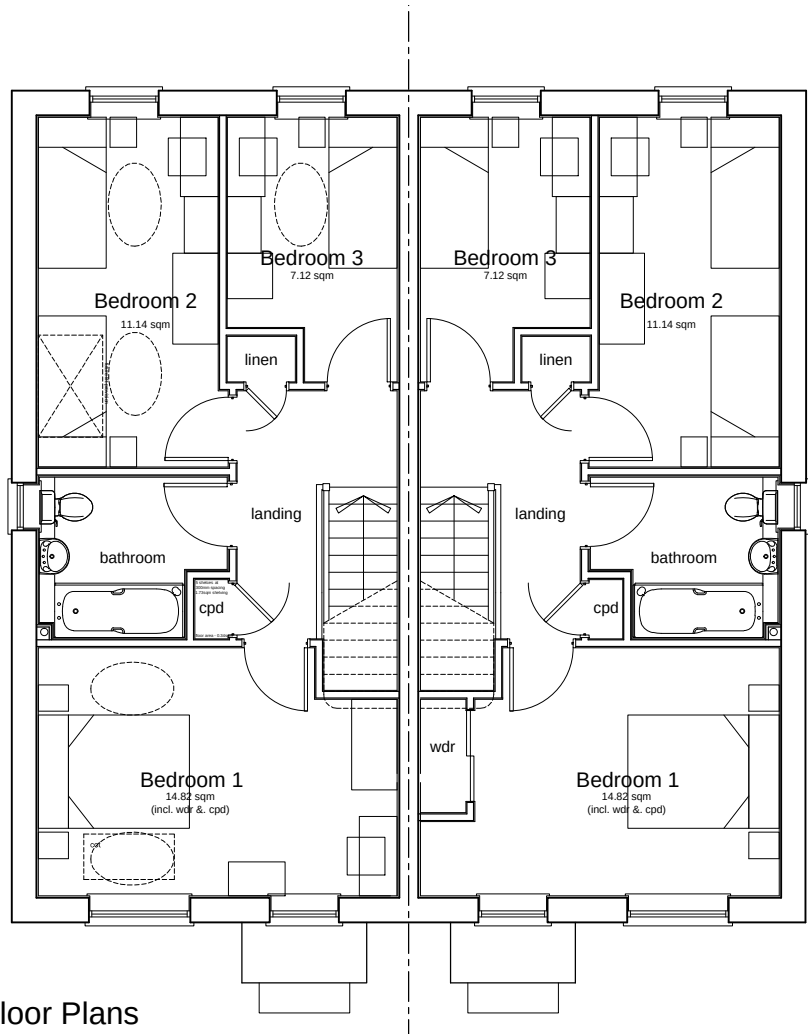
First Floor Plans
