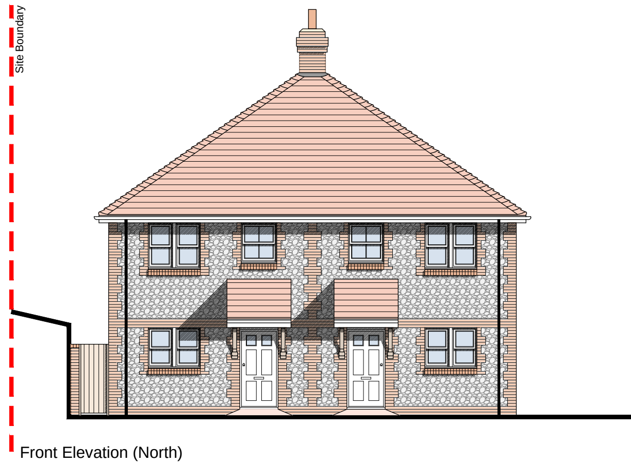
Front Elevation (North)
