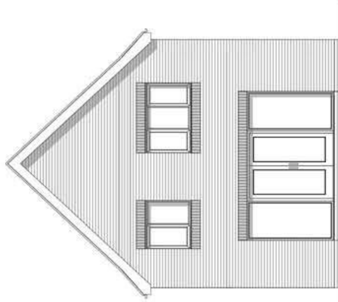
Rear Elevation
