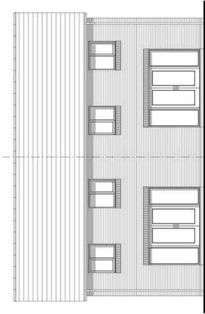
Rear Elevation
