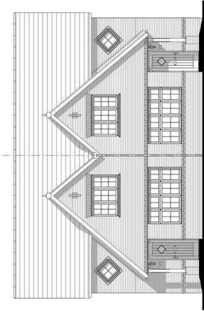
Front Elevation
