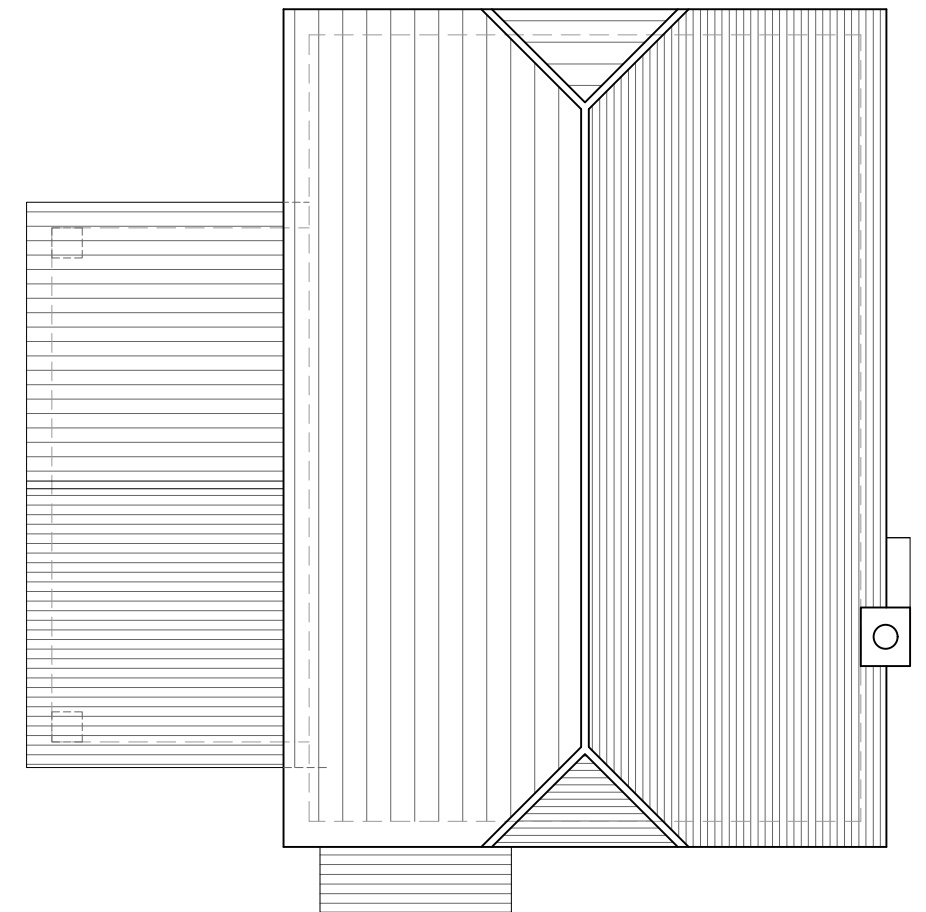
03 House Type A - Roof Plan - 4B/6P 1:100
