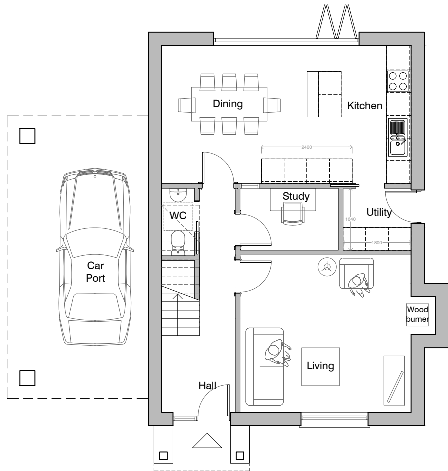
01 House Type A - Ground Floor - 4B/6P 1:100
