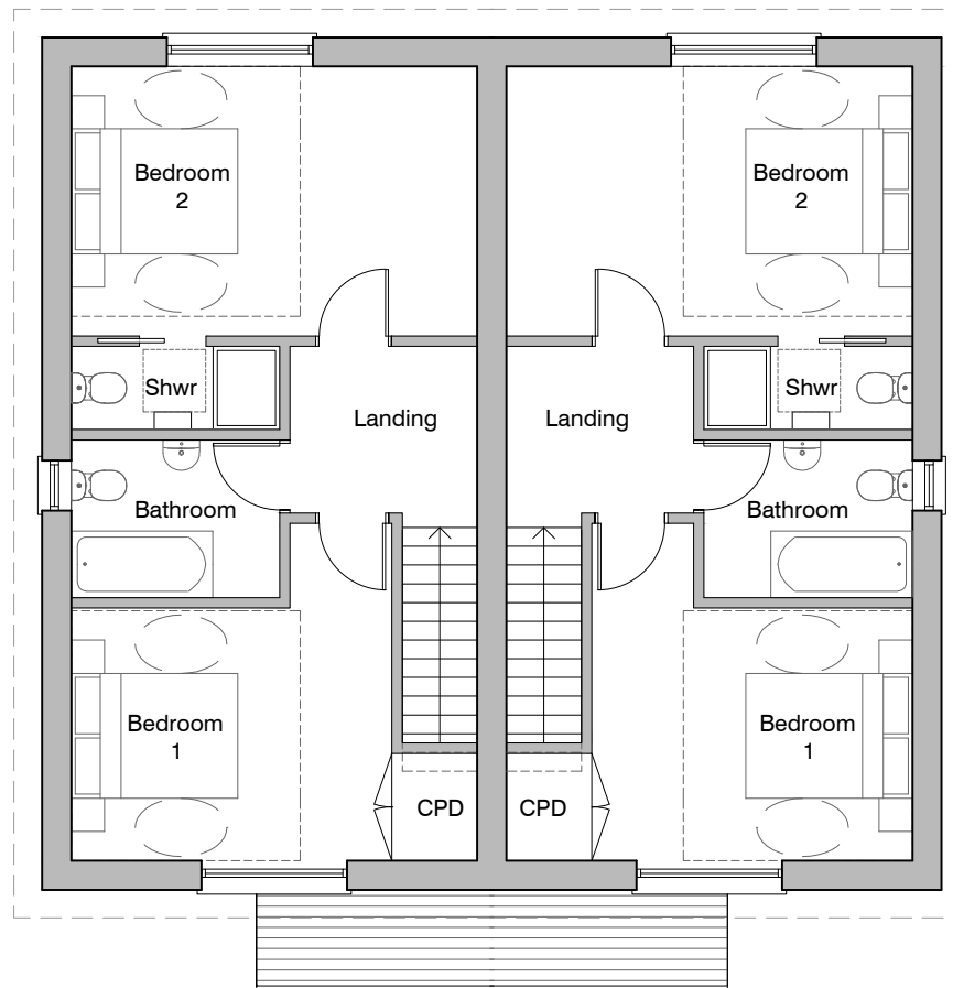
02 House Type C - First Floor - 2B/4P 1:100 Total House: 92.8 sqm First Floor: 46.4 sqm
