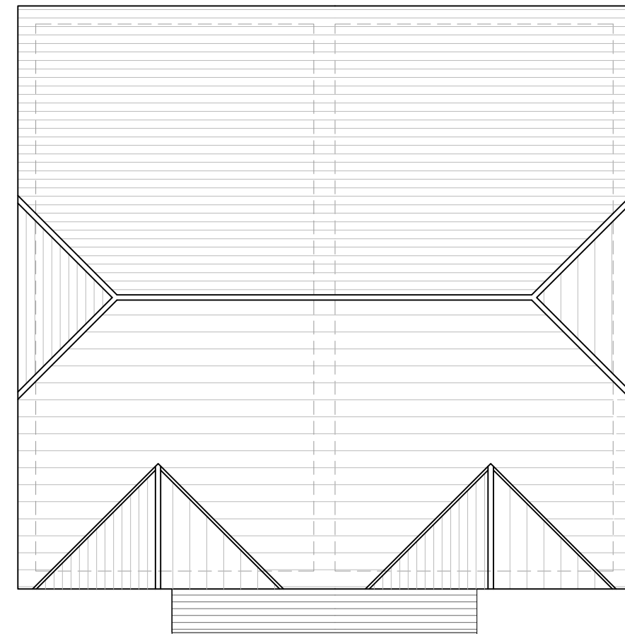
03 House Type C - Roof Plan - 2B/4P 1:100 Total House: 92.8 sqm
