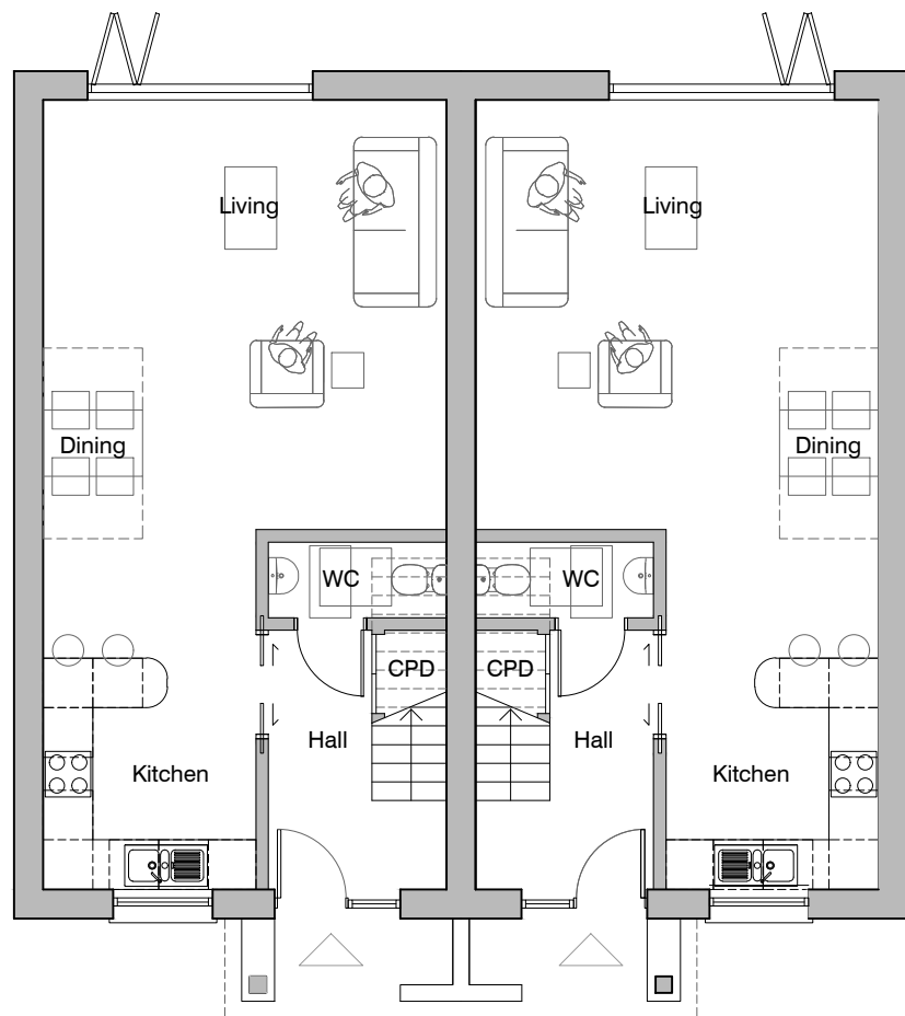
01 House Type C - Ground Floor - 2B/4P 1:100 Total House: 92.8 sqm Ground Floor: 46.4 sqm
