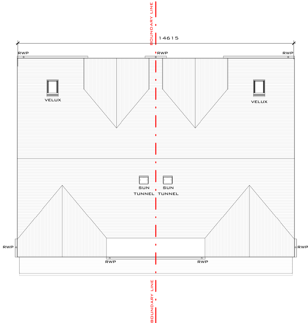
PROPOSED ROOF PLAN 1 : 100 @ A3
