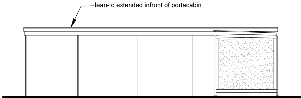
North Elevation 1:100@A3
