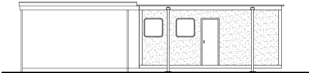
East Elevation 1:100@A3
