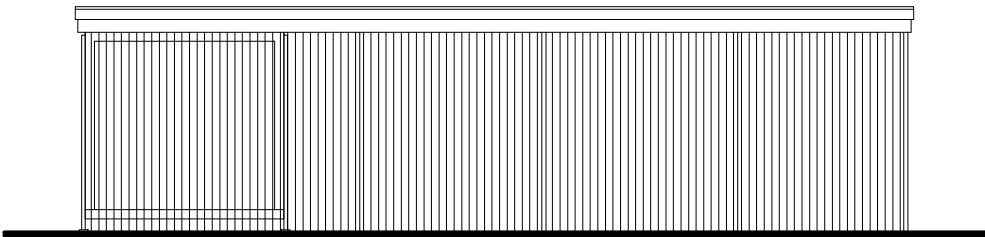
South Elevation 1:100@A3
