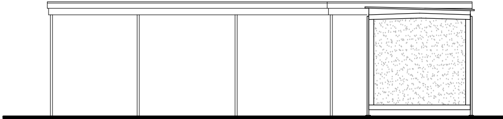
North Elevation 1:100@A3
