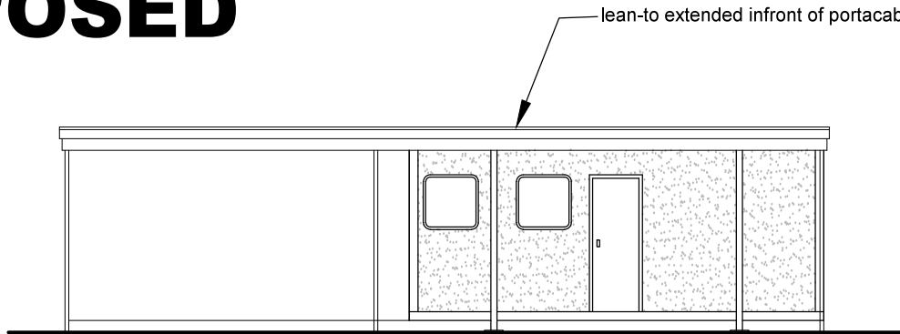
East Elevation 1:100@A3
